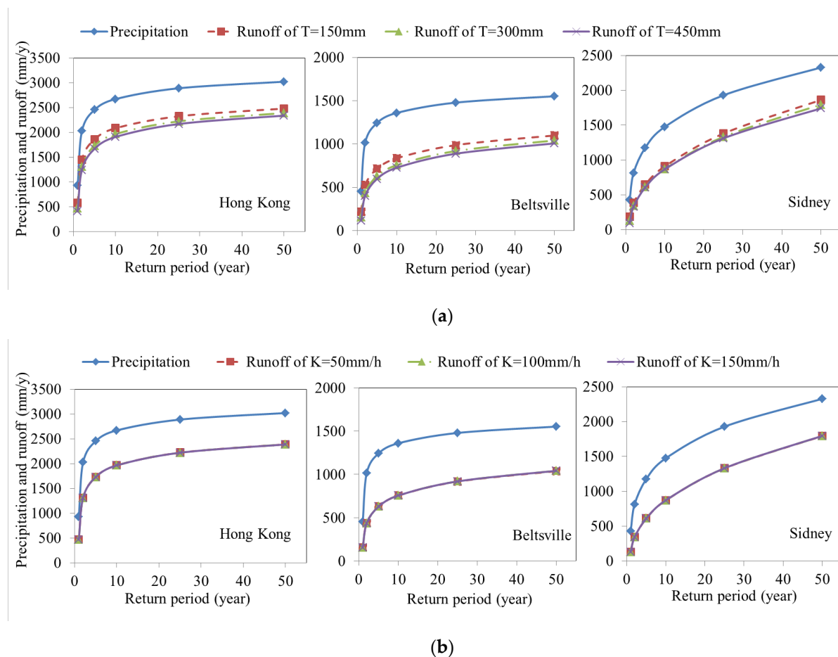
Figure 7. Average runoff of various green roofs differing in (a) soil thickness (T) and (b) soil hydraulic conductivity (K). The conductivity in (a) is 100 mm/h, and the thickness in (b) is 300 mm.
