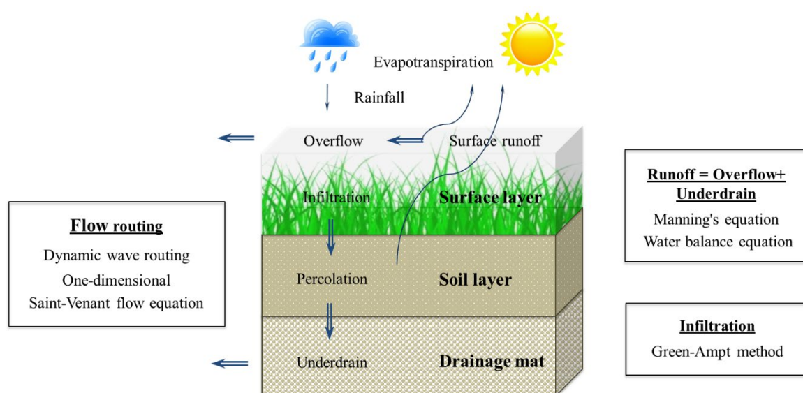
Figure 1. Conceptual model of green roof in SWMM. Modified from Chui et al. [28].
