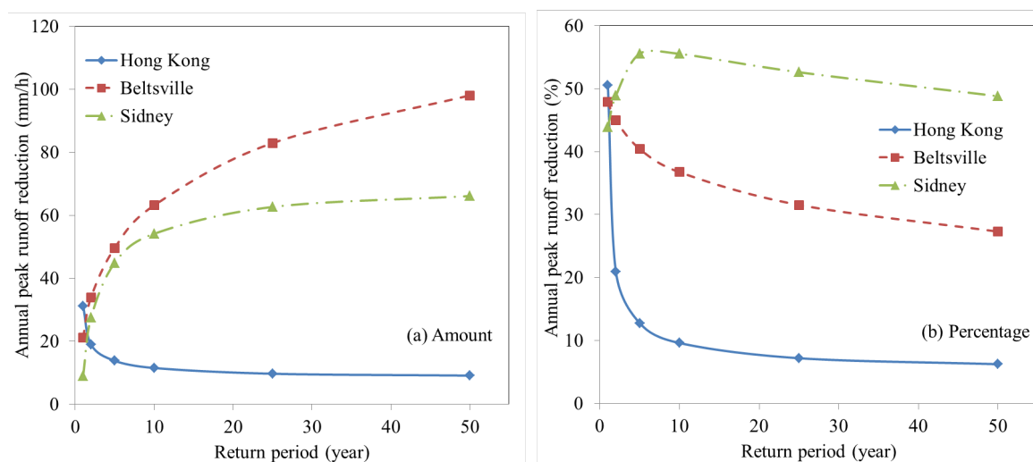
Figure 4. Annual peak runoff reduction during storms with different return periods, given in terms of (a) amount and (b) percentage.
