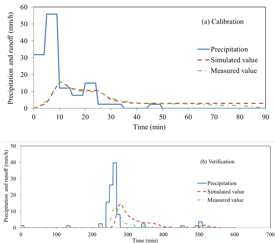
Figure 2. Simulated and measured values of green roof runoff during model (a) calibration and (b) verification.
