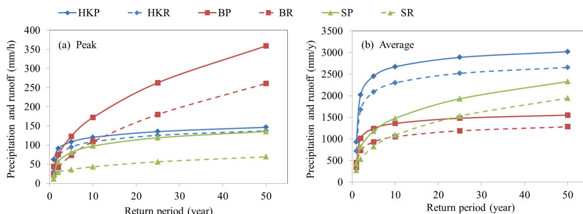
Figure 3. Precipitation (P) and green roof runoff (R) in storms with different return periods. Figure 3(a) and (b) show the peak and average values, respectively. HK, B and S stand for Hong Kong, Beltsville and Sidney, respectively.
