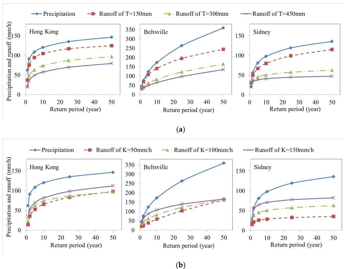
Figure 6. Peak runoff of various green roofs differing in (a) soil thickness (T) and (b) soil hydraulic conductivity (K). The conductivity in (a) is 100 mm/h, and the thickness in (b) is 300 mm.
