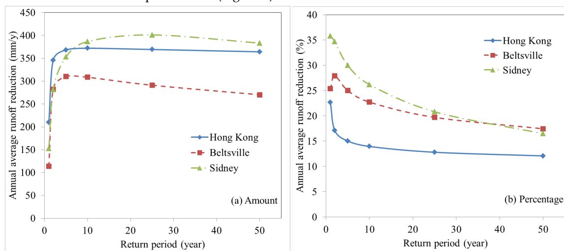
Figure 5. Annual average runoff reduction during storms with different return periods, given in terms of (a) amount and (b) percentage.
