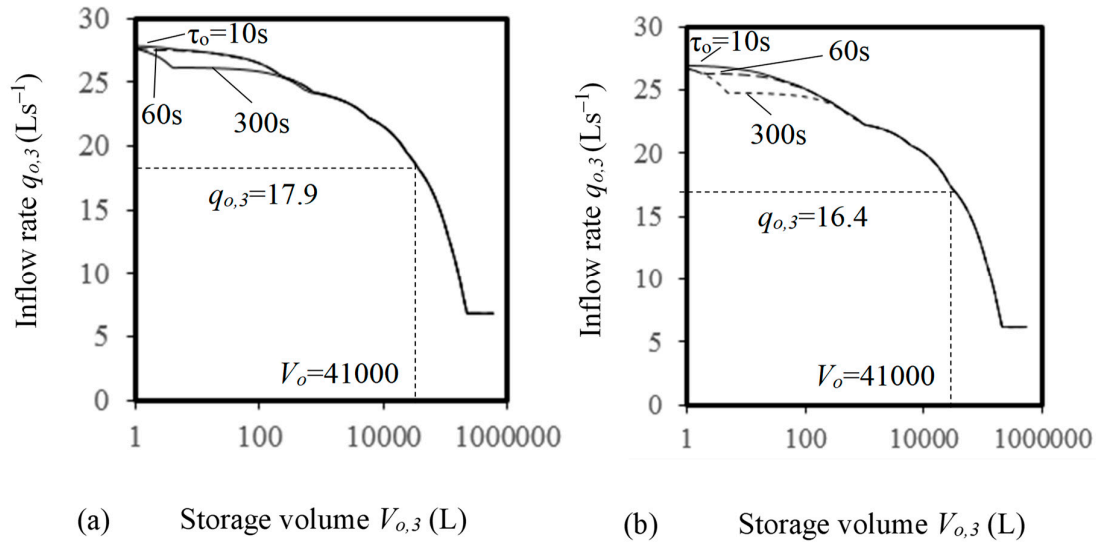
Figure 6. Solutions of inflow rate and storage volume at Zone 3 (a) for the maximum demand time series in Figure 5a and (b) for the minimum demand time series in Figure 5b.
