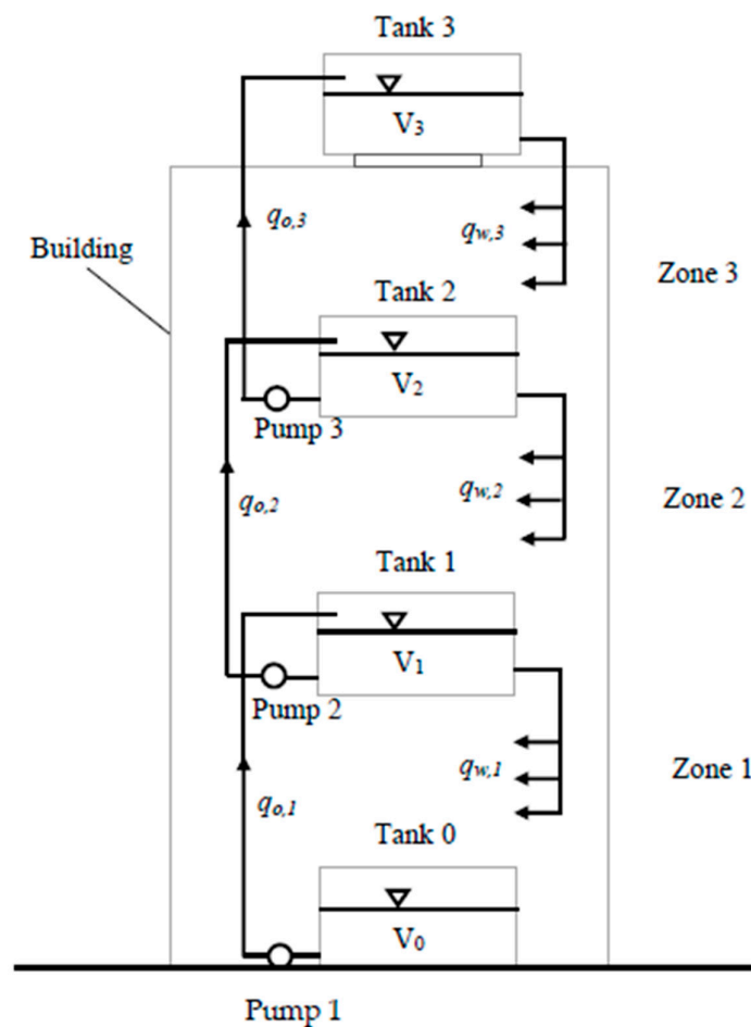
Figure 1. A cascade water supply system in a skyscraper.
