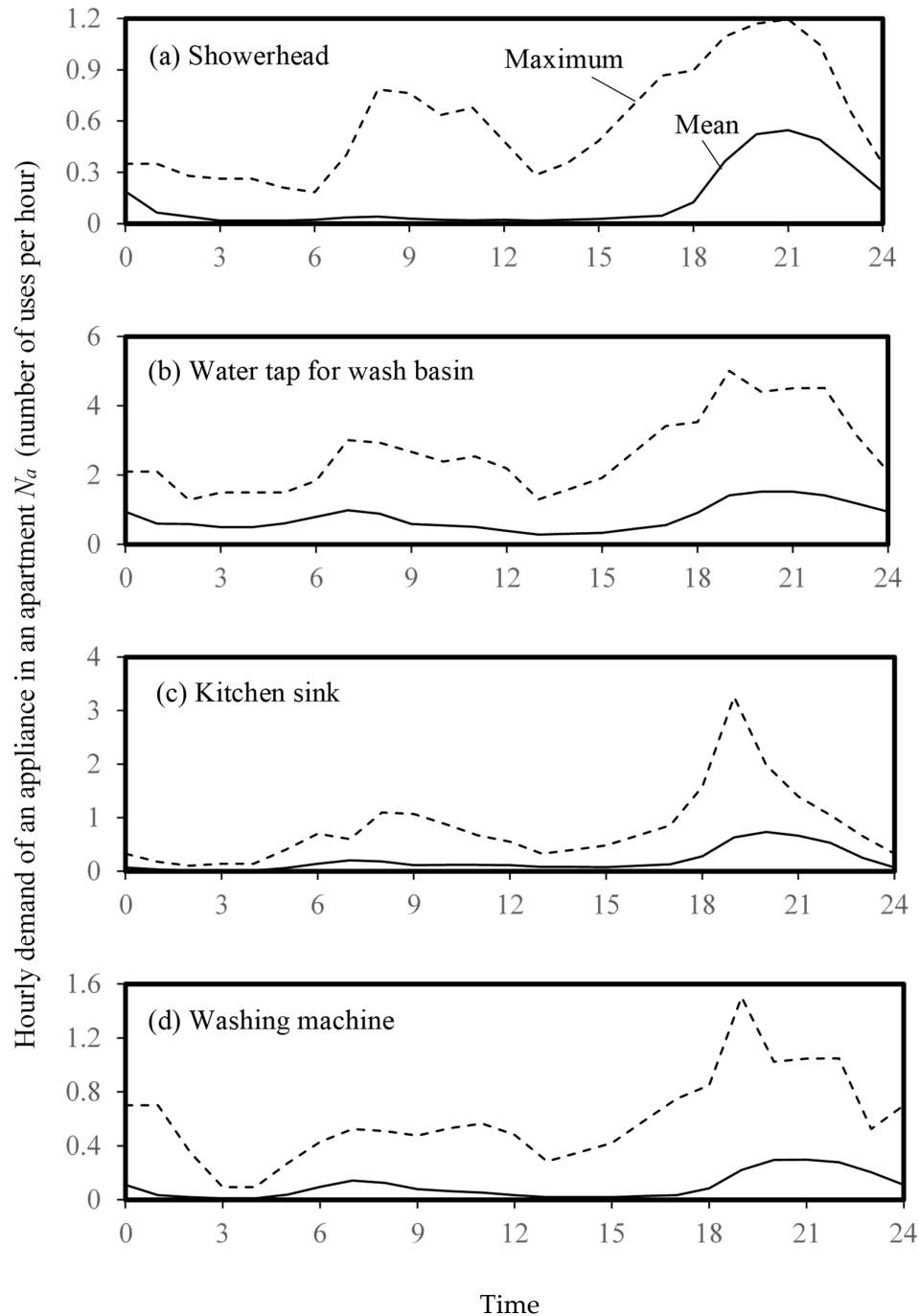
Figure 4. Hourly demand of each type of appliances in an apartment: (a) showerhead; (b) wash basin; (c) kitchen sink; (d) washing machine [16,17].
