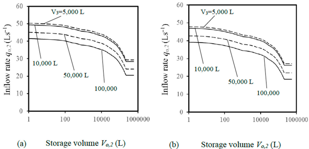
Figure 8. Solutions of inflow rate and storage volume at Zone 2 (a) for the maximum demand time series in Figure 5a and (b) for the minimum demand time series in Figure 5b.
