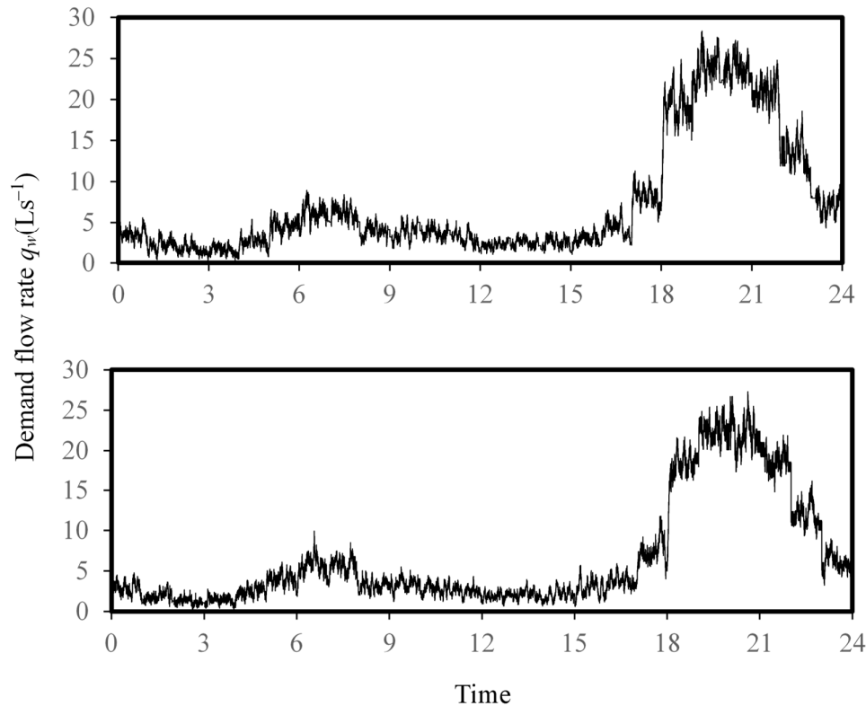
Figure 5. Total demand flow rates: (a) maximum daily consumption ( 590.0 \text{ m}^3\text{d}^{-1} ); (b) minimum daily consumption ( 534.8 \text{ m}^3\text{d}^{-1} ).
