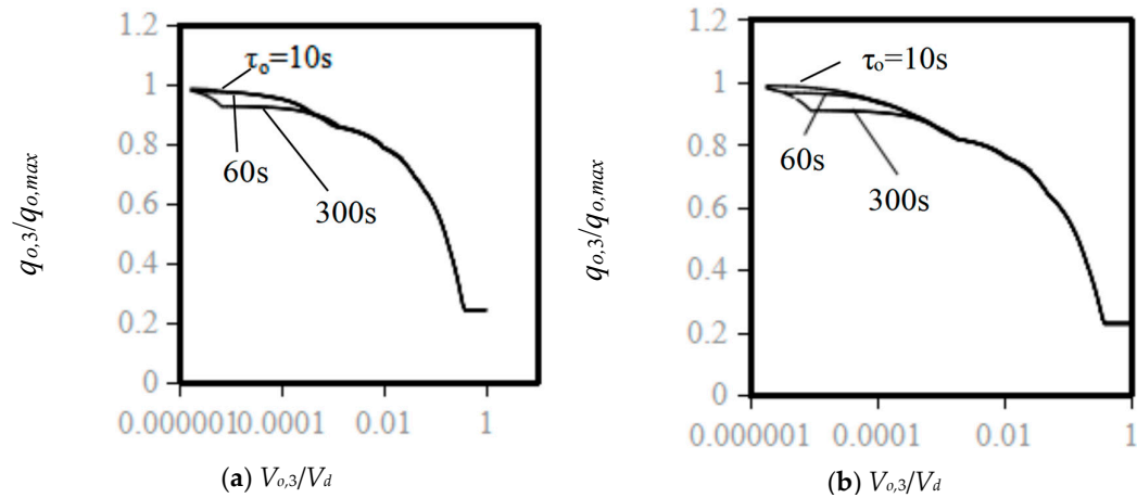
Figure 7. Solutions of normalized inflow rate and storage volume at Zone 3 (a) for the maximum demand time series in Figure 5a and (b) for the minimum demand time series in Figure 5b.
