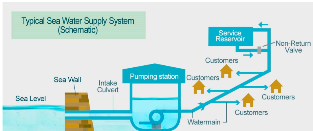
Figure 2. The schematic diagram of a typical sea water supply system in Hong Kong [13].
