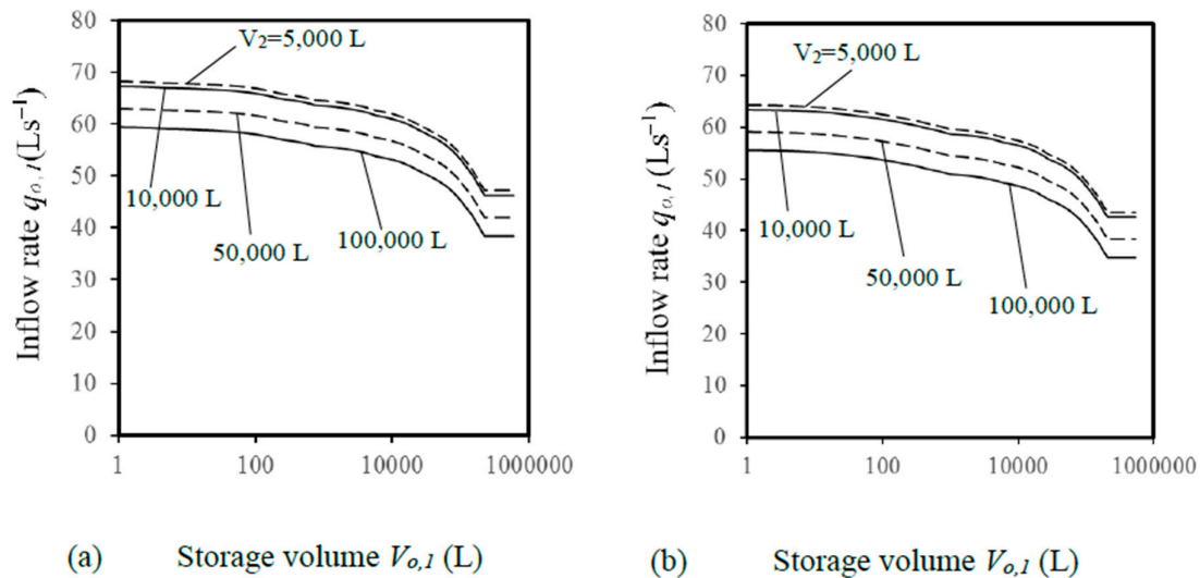
Figure 9. Solutions of inflow rate and storage volume at Zone 1 (a) for the maximum demand time series in Figure 5a and (b) for the minimum demand time series in Figure 5b.
