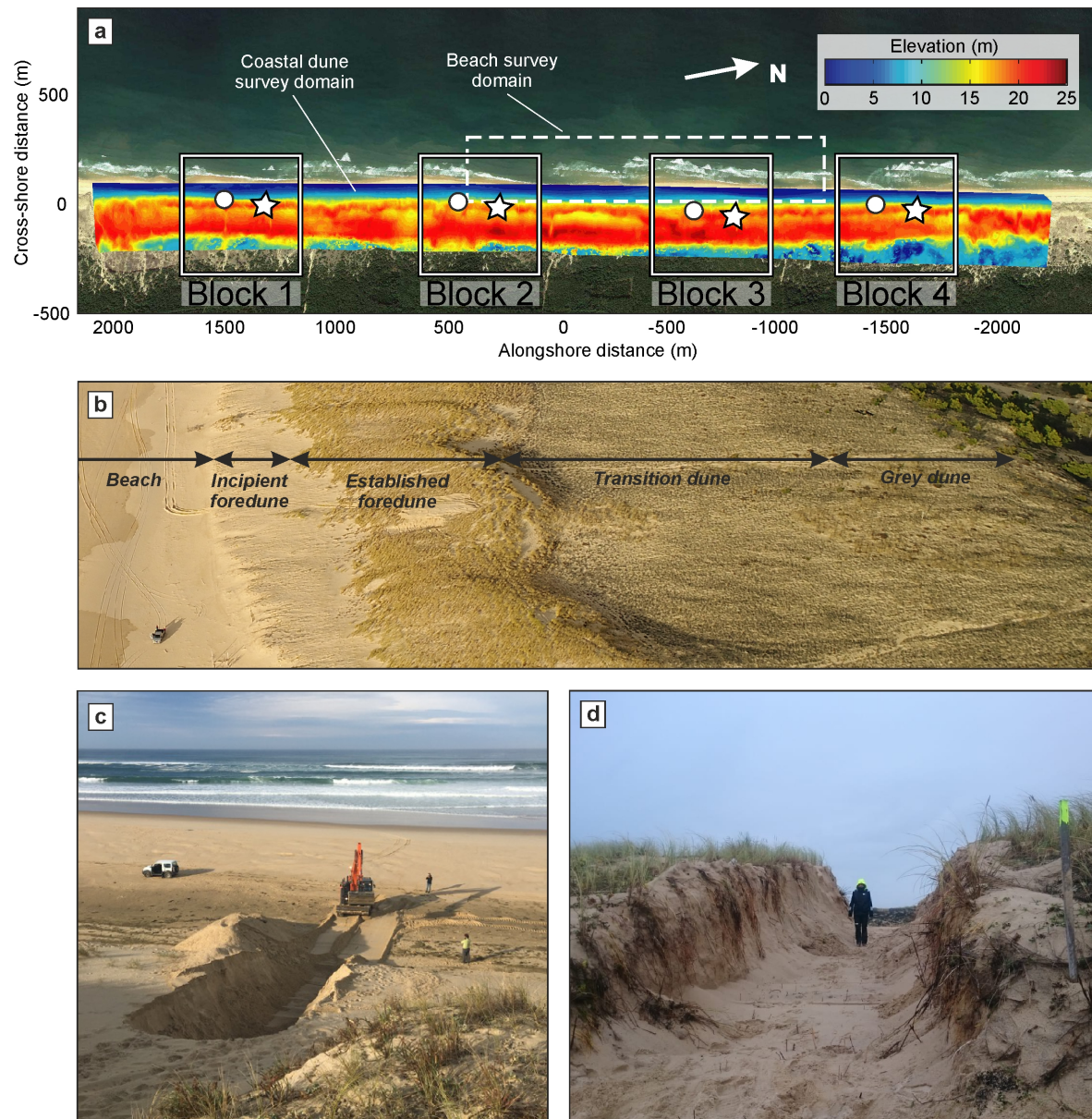
Figure 5. (a) Truc Vert experimental site. A digital surface model (DSM) of the coastal dune system inferred from photogrammetry using a low-cost unmanned aerial vehicle (UAV) is coloured, and the dashed white rectangle shows the beach area which is surveyed semi-monthly with a differential global positioning system (DGPS)-equipped ATV. The solid rectangles indicate the experimental blocks (1-4) where notches were excavated in the incipient foredune (circles) and in the established foredune (stars). (b) Truc Vert beach landscape with indication of the typical coastal dune compartments and with the 4-wheel drive making the scale. (c) Incipient foredune notch excavated on 5 November 2018 (Ph. B. Castelle). (d) Established foredune 2.5-m-deep notch with Q. Laporte-Fauret made the scale (Ph. V. Marieu).
