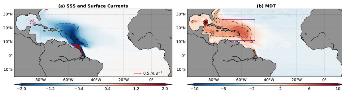
Figure 5. Amazon runoff contribution to the mean-state of oceanic surface variables: (a) SSS (PSU, color) and surface currents ( \text{m}\cdot\text{s}^{-1} , arrows) and (b) Mean Dynamic Topography (cm). The purple rectangle is the box used to compute area averaged diagnostics. Averages have been performed over the period 1993–2015.
