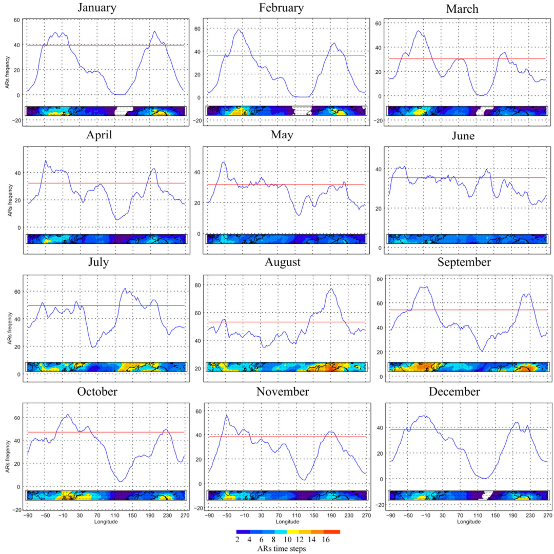
Figure S1. AR frequency over the area between 55° and 65° N over the period 1997–2014: The blue line represents the number of ARs for every longitude and the box embedded in the plot shows the spatial distribution of the ARs. Reddish colours represent areas with higher AR frequency and bluish colours those with lower. The red lines depict the 75th percentile of the distribution.
