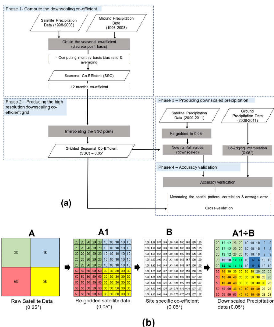
Figure 3. (a) Overall methodology. (b) Methodological flowchart of the spatial downscaling process—generating the high resolution precipitation data.
