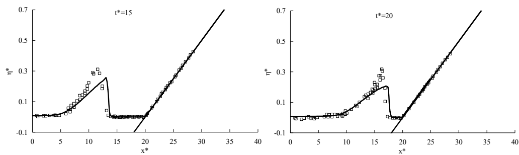
Figure 3. Run-up and run-down of H_w/h_0 = 0.0185 non-breaking solitary wave on a 1:19.85 sloping beach.
