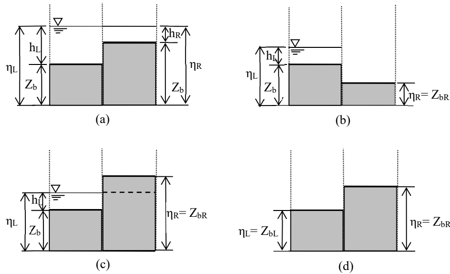
Figure 1. Schematic diagram of wet-dry edges.
