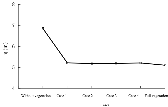
Figure 16. The comparison of maximum run-up heights.
