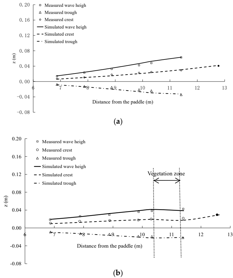
Figure 6. Comparison of measured and calculated wave crests, heights, and troughs. (a) Case without vegetation, (b) Case with full vegetation.
