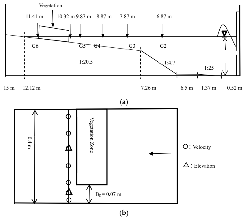
Figure 5. Experimental setup of wave flume. (a) Longitudinal section, (b) plan view of vegetation zone and measurement points.
