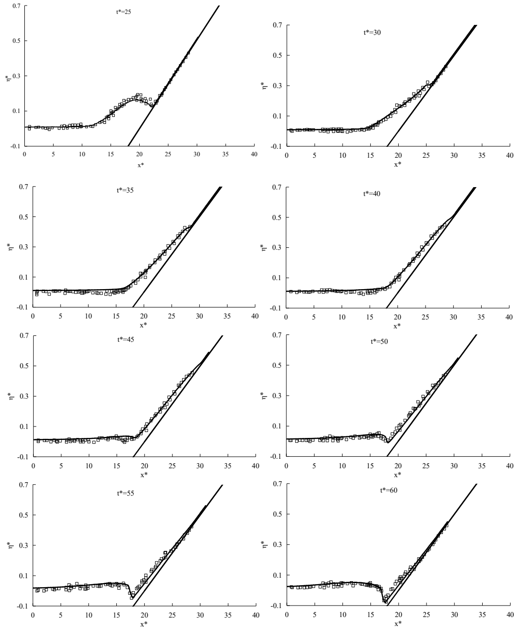
Figure 4. Run-up and run-down of H_w/h_0 = 0.3 breaking solitary wave on a 1:19.85 sloping beach.
