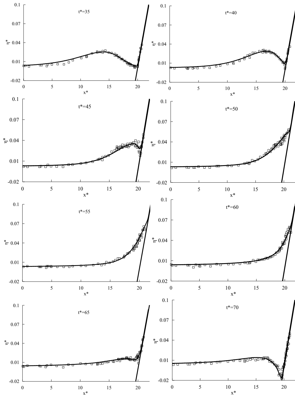
Figure 3. Run-up and run-down of H_w/h_0 = 0.0185 non-breaking solitary wave on a 1:19.85 sloping beach.
