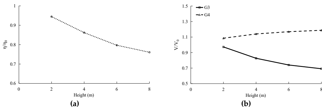
Figure 18. Variation of normalized run-up heights and normalized peak flow velocities at G3 and G4 with different densities of pure P. odoratissimus . (a) The normalized run-up heights, (b) The normalized peak flow velocities.
