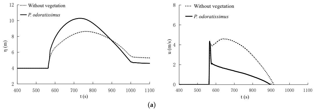
Figure 12. Flow structure in Case 1 at different times ((a) T = 600 s, (b) T = 660 s, (c) T = 700 s).
