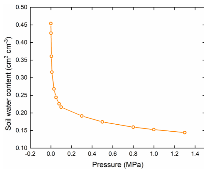
Figure S1. Soil water retention curve of the homogenous soil in the WTDPD.
