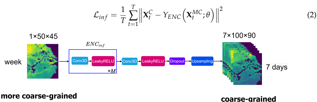
Figure 5. Illustration of super-resolution pretext task.
