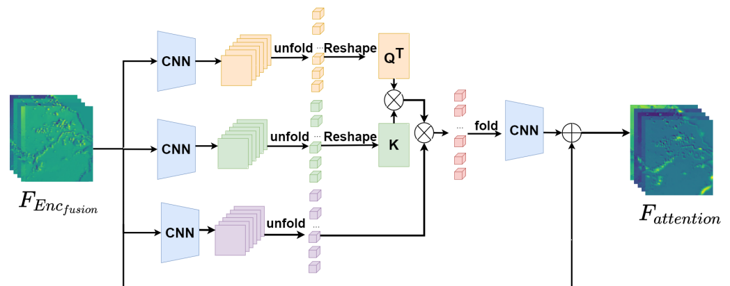
Figure 7. Illustration of 3D-patch-wise self-attention convolutional module, where the input F_{Encfusion} are fusion features generated by the spatiotemporal super-resolution pretext task. The unfold operation uses a sliding window to decompose and combine feature maps into patches, and the fold operation is used to recombine patches into feature maps F_{attention} .
