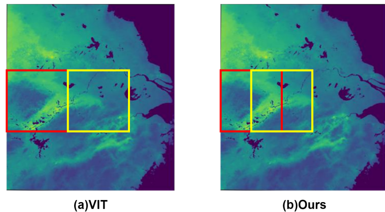
Figure 6. (a) The VIT divides images into blocks without overlap while pollutants affect spatial structure. (b) Our self-attention models overlap the chunks, which retains the structure and enhances local correlation.
