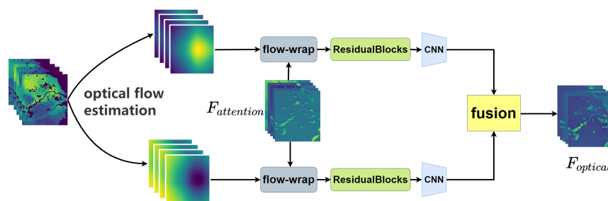
Figure 10. The optical flow map is combined with the feature map F_{attention} from the attention mechanism. Furthermore, a two-way propagation network then generates separate feature maps, which are fused into F_{optical} .
