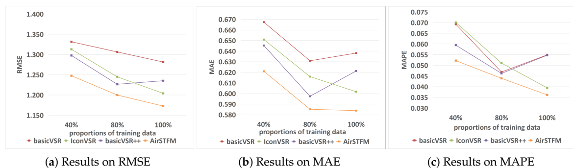
Figure 12. Results compared to baseline methods for different training set sizes.
