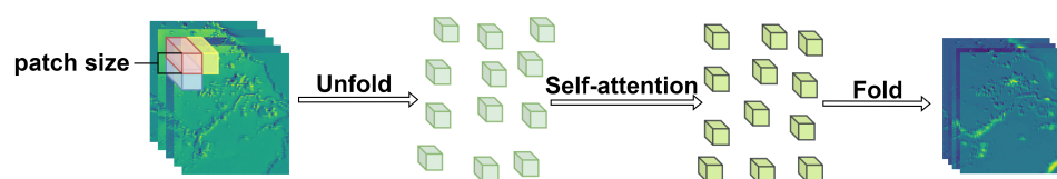
Figure 8. Unfolding the convolved spatial-temporal diffusion feature maps.
