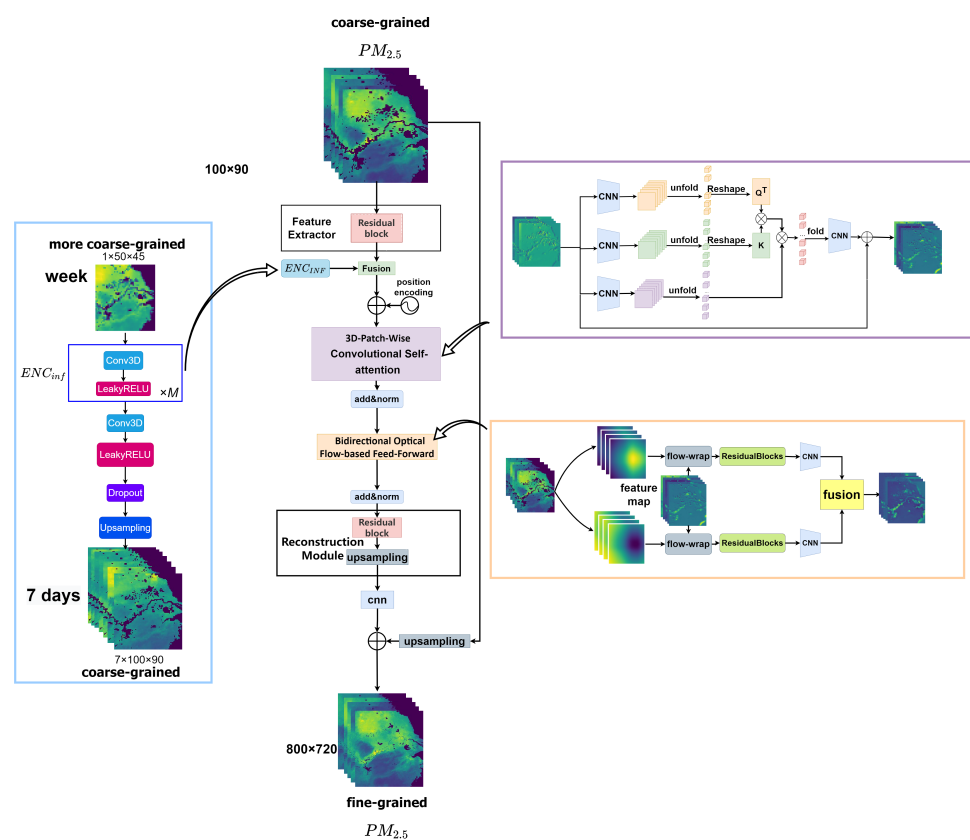
Figure 4. The framework of AirSTFM, which contains three modules, a 3D-patch-wise convolutional self-attention module, bidirectional optical flow-based feed-forward module, and a spatial–temporal super-resolution inference network, for extracting high-level contaminant semantic information using a pretext task.
