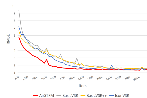
Figure 15. Convergence speed comparison of different models.
