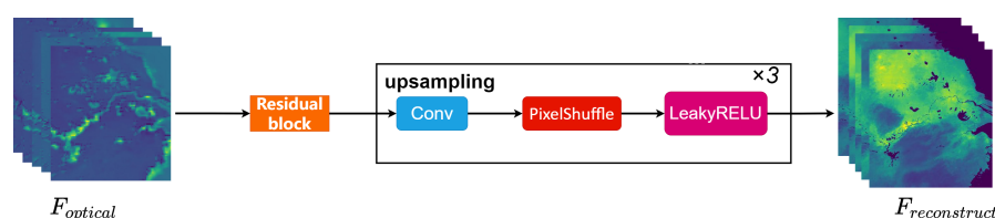
Figure 11. The feature maps obtained from the optical flow were residualized and upsampled to obtain fine-grained spatial and temporal distributions of the feature contamination.
