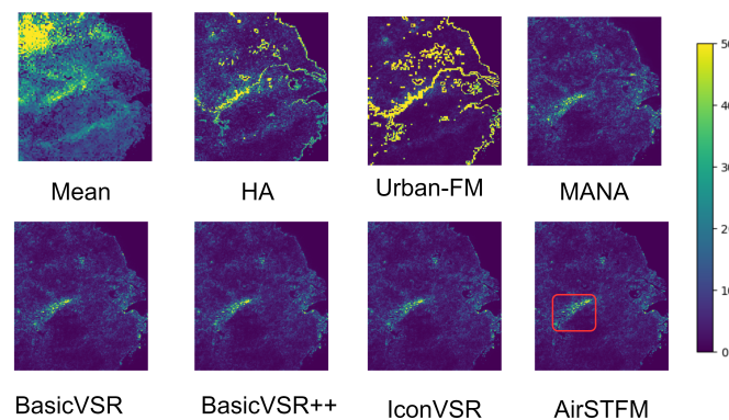
Figure 16. Visualization of the difference between inferred and actual values.
