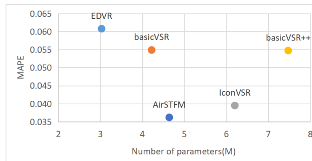
Figure 14. Model parameters' comparison.
