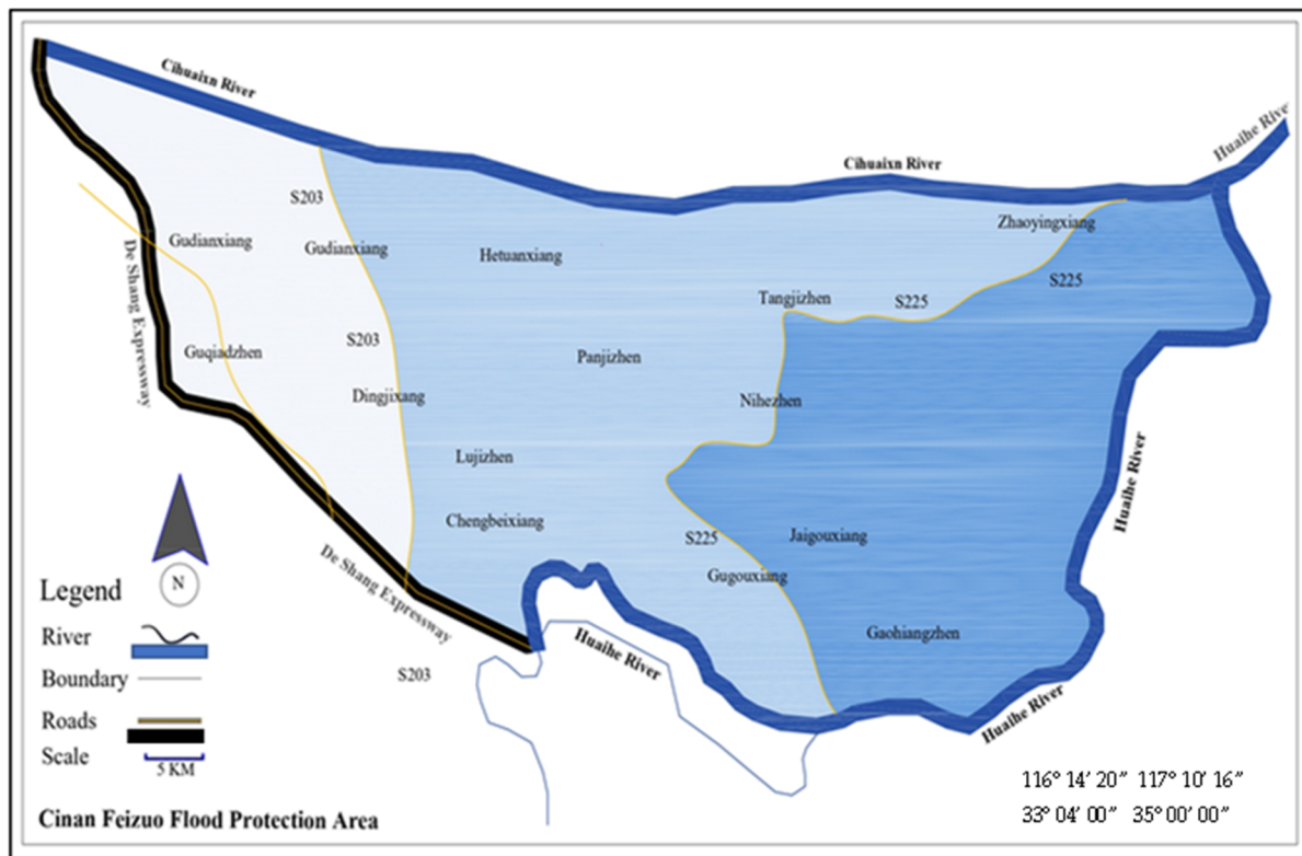
Figure 1. Huaihe River and Cinan Fiezuo flood protection area: topographic elevation, drainage water boundaries ( upper ), and Cinan Feizuo flood protection area with side artificial Cihuaixin channel and Huaihe River ( lower ).
