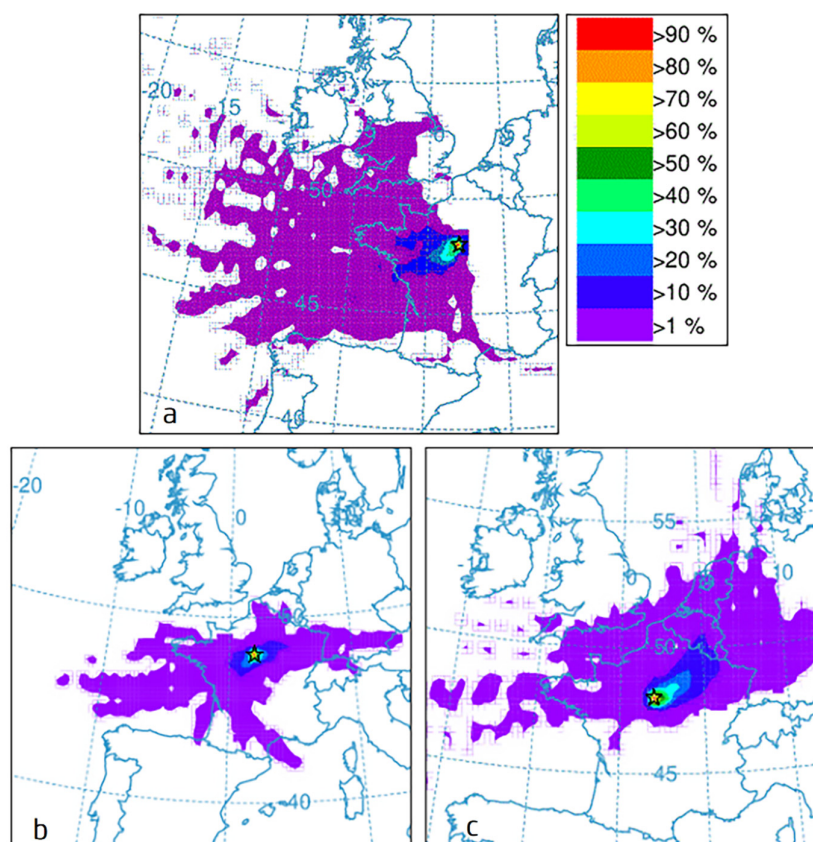
Figure 9. Results of HYSPLIT 24 h back trajectory frequencies before (a), during (b), and after (c) the lockdown. The star represents the location of the measurement site. Height: 500 m above the ground level; frequency grid resolution: 0.5 \times 0.5^\circ .
