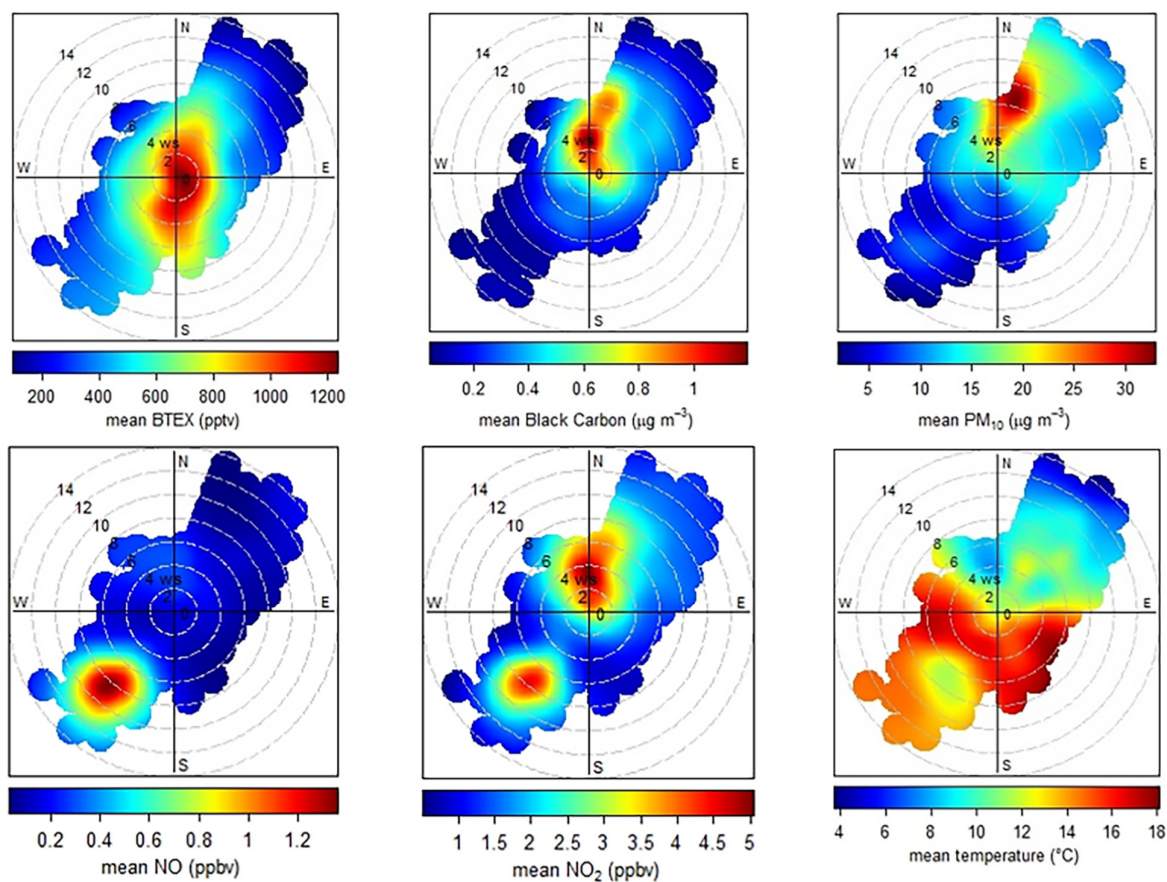
Figure 8. Polar plots of BTEX, NO, NO 2 , O 3 , PM 10 , BC, and temperature (T) for lockdown (from 17 Mar to 10 May); ws = wind speed (m s −1 ).
