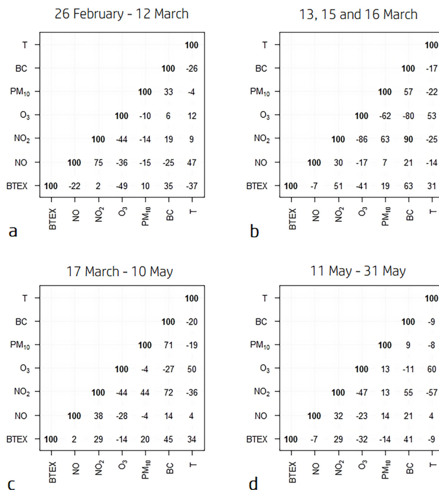
Figure 7. Correlation coefficient in percentage between BTEX, NO, NO 2 , O 3 , PM 10 , BC, and temperature (T) for each period ((a) before; (b) declared; (c) during; (d) after lockdown).
