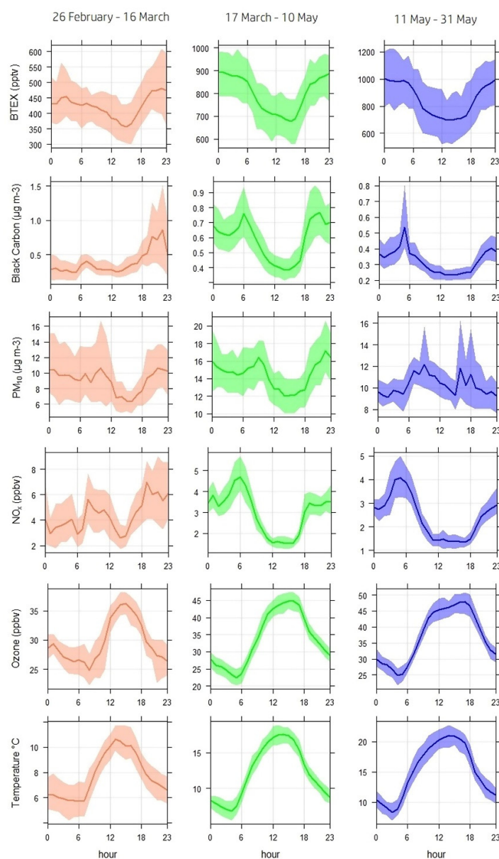
Figure 3. Diurnal variations in BTEX, BC, PM 10 , NO x , O 3 , and temperature before, during and after lockdown. The shaded area represents 95% confidence interval in mean.
