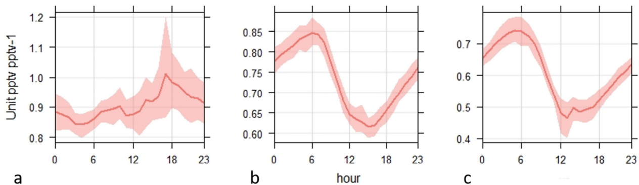
Figure 6. Diurnal variations in MP/E ratio (a) before, (b) during, and (c) after the lockdown.
