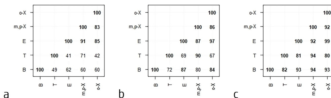
Figure 4. Correlation coefficients in percentage between benzene, toluene, ethylbenzene, m,p-xylene and o-xylene (a) before, (b) during, and (c) after the lockdown.
