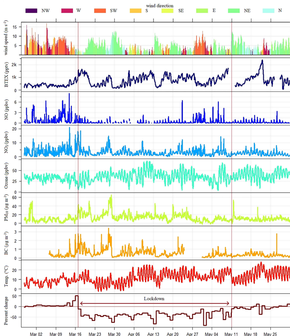
Figure 2. Time series of hourly BTEX (pptv, y axis of BTEX 1k = 1 \times 10^3 ), NO (ppbv), NO 2 (ppbv), O 3 (ppbv), PM 10 ( \mu\text{g m}^{-3} ), black carbon ( \mu\text{g m}^{-3} ), and temperature ( ^{\circ}\text{C} ) in Orléans during the studied period, with daily “percent change in the grocery and pharmacy”, and meteorological parameters (wind speed in \text{m s}^{-1} , wind direction in a color-coded way).
