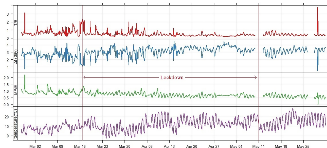
Figure 5. Variation of toluene/benzene (T/B), photochemical age of the air ( \Delta t ), m, p-xylene/ethylbenzene (MP/E) concentration ratios and temperature in the observation site during the entire measurement period.
