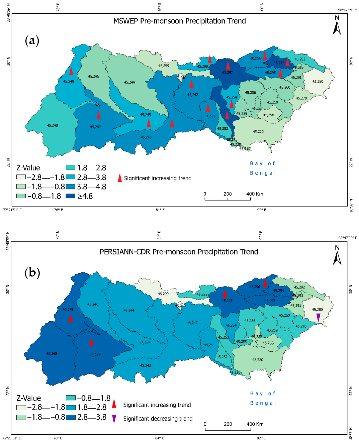
Figure 5. Pre-monsoon precipitation trend for (a) MSWEP and (b) PERSIANN-CDR. Red color upright triangle indicates a significant increasing trend ( p < 0.05 ), and a purple color downright triangle indicates significant decreasing trend.
