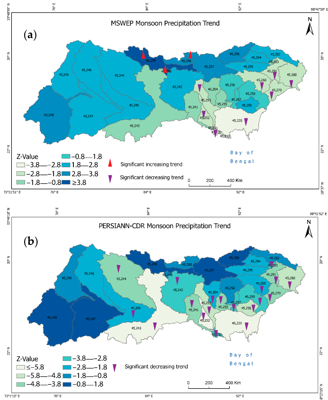
Figure 6. Monsoon precipitation trend for (a) MSWEP and (b) PERSIANN-CDR. Red color upright triangle indicates a significant increasing trend ( p < 0.05 ), and a purple color downright triangle indicates significant decreasing trend.
