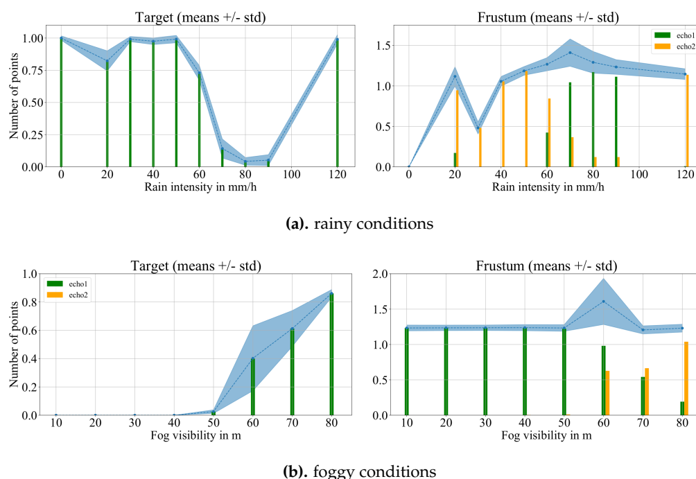
Figure 15. Results from VLP-32 with multi-echo labels.
