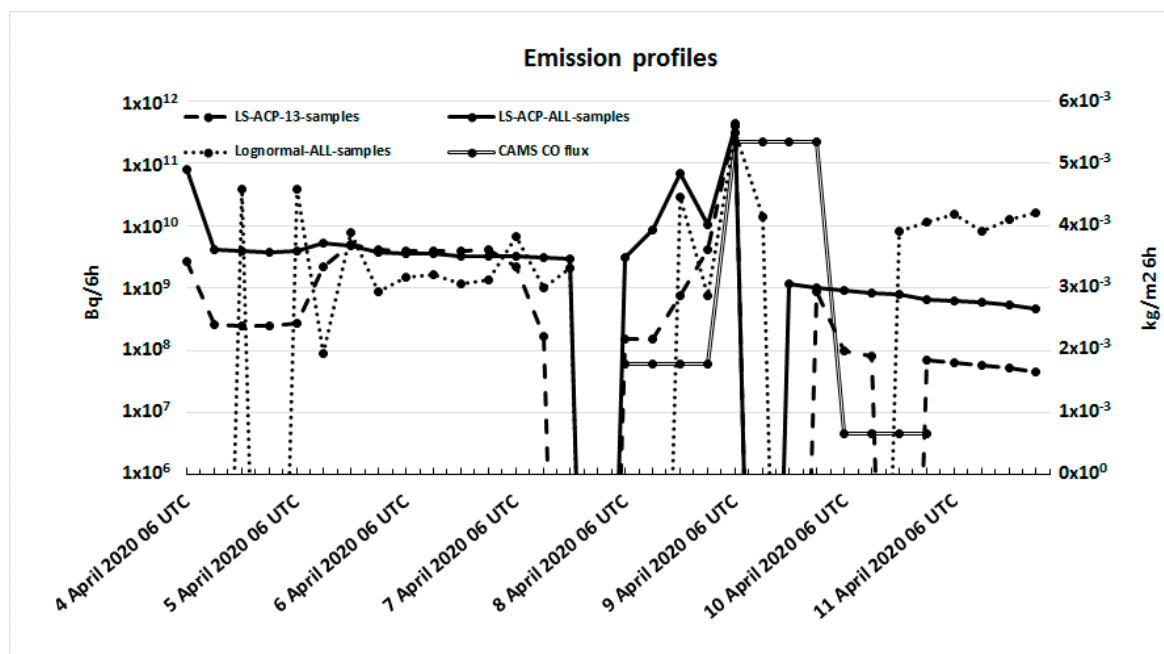
Figure 5. Cs-137 mission profiles (Bq/6 h) for the period 4 to 12 April resulting from the LS-ACP and the lognormal approaches as well as the CAMS CO emission flux ( \text{kg}/\text{m}^2 6 h) for 8 to 11 April. Source location was constraint to 1000–3000 m a.g.l. in the vertical and nine grid cells centered on the fire location according to CAMS. Zero emission values are not shown. Filled circles indicate the released activity, the total flux respectively, at the end of each six-hour period.
