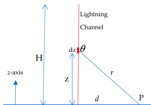
Figure 1. Geometry relevant to the calculation of electromagnetic fields from a return stroke.
