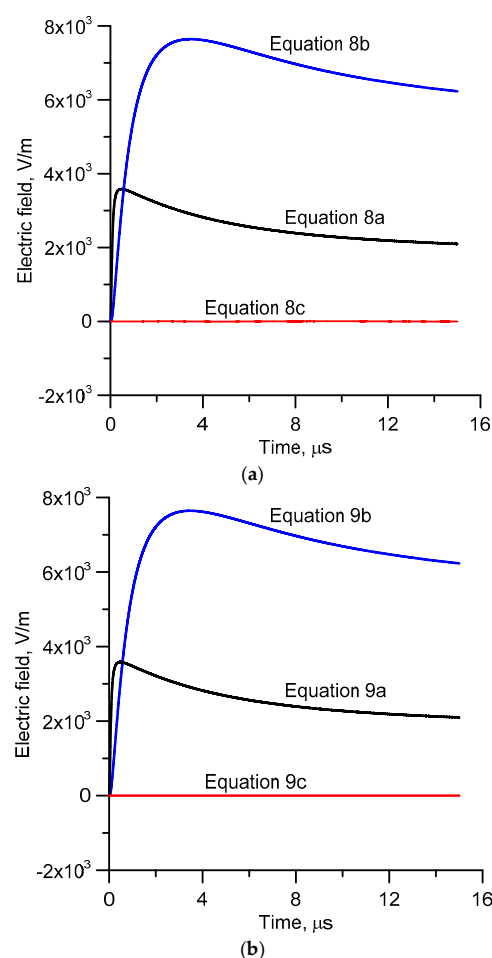
Figure A2. Plot of the field components associated with (a) Equation (8a–c) and (b) Equation (9a–c). The electric field is calculated at 100 m from the strike point of a lightning return stroke simulated by the transmission line model. The current at the channel base is represented by the analytical expression given by Nucci et al. [17] to represent subsequent return strokes. The return stroke speed used in the calculation is 1.5 \times 10^8 m/s.
