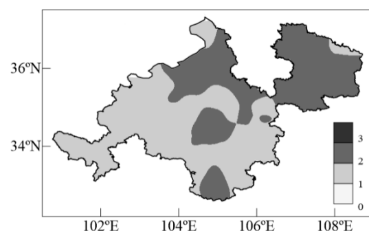
Figure 2. Average number of drought processes from 1960 to 2017 (units: numbers/per year).
