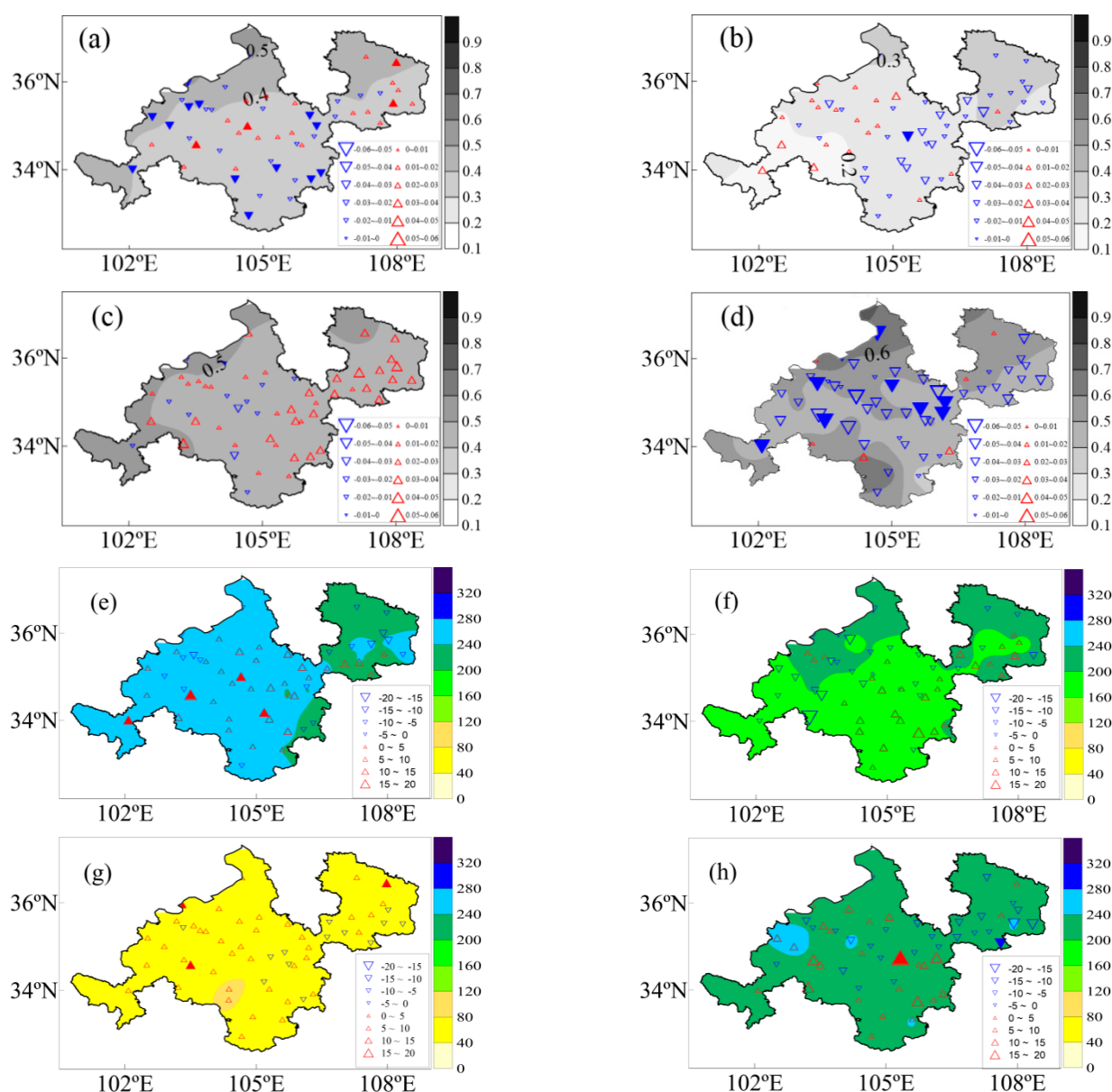
Figure 8. Average precipitation heterogeneity and its trend in each season. ((a–d) are PCD in spring, summer, autumn, and winter, respectively; (e–h) are PCP in spring, summer, autumn, and winter, respectively; solid indicates the trend is significant at the 0.05 level based on the Student's t -test.).
