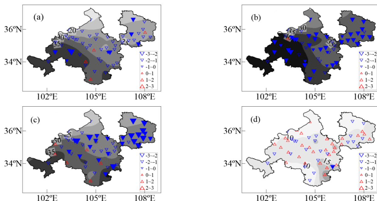
Figure 9. Average days with light and moderate rain and its trend in each season ((a–d) are spring, summer, autumn, and winter, respectively; solid indicates the trend is significant at the 0.05 level based on the Student’s t -test).
