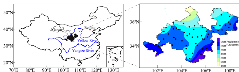
Figure 1. Distribution of annual average precipitation (unit: mm) and the location of the study area, meteorological stations (black spots).
