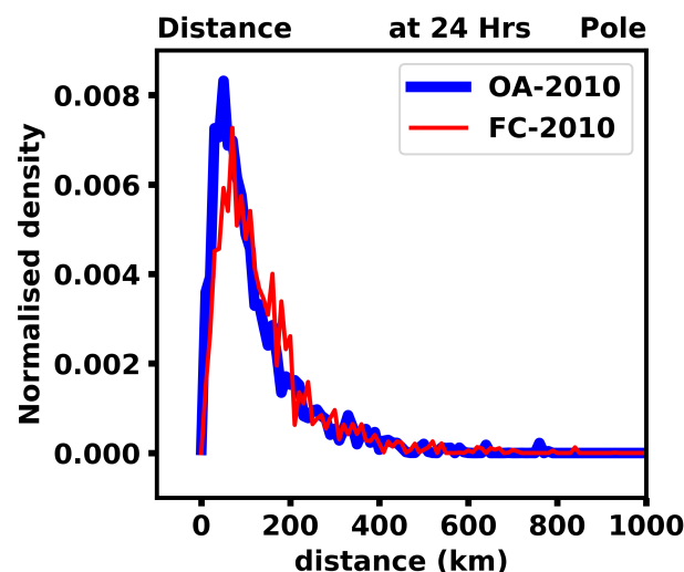
Figure 2. Probability Density Function (PDF) of spherical distance between the real and simulated balloon trajectories during the Concordiasi campaign with the ECMWF 2010 operational analyses (blue), and forecasts (red).
