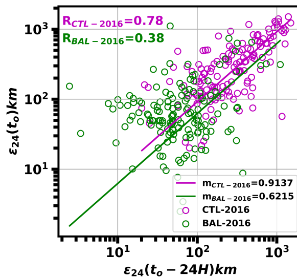
Figure 11. Scatterplot of the error in position after 24 h (vertical axis), as a function of the error in the trajectory started 24 h earlier (horizontal axis), for simulations using CTL-2016 (purple) and for those using BAL-2016 (green). Note the logarithmic axes. The linear correlation coefficients ( R ) and slope of the regression line ( m ) in log-log space are provided in the figure.
