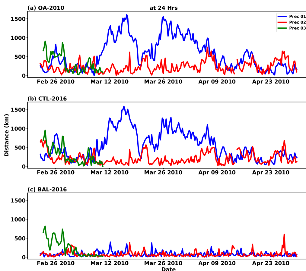
Figure 10. Time series of spherical distance between the real and simulated balloon positions after 24 h of simulation, for the three PreConcordiasi balloons. The simulated trajectories are calculated using the OA-2010 (top panel), CTL-2016 (middle panel) and BAL-2016 (bottom panel) IFS setups.
