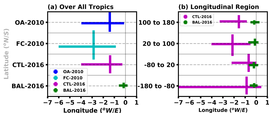
Figure 9. Summary of the balloon trajectory errors in longitudes (x-axis) and latitudes (y-axis) after 24 h of simulation for the different IFS setups. The left panel displays the errors statistics obtained over the whole tropics, while the right panel displays those errors in different longitude ranges for the CTL-2016 and BAL-2016 setup. Shown are the 25th–75th interquartile error spreads both in longitude and latitude. The two spreads cross at the median longitudinal and latitudinal errors. The latitude scale on the y-axis is represented by horizontal (either dotted or solid) lines that are plotted every degree. Dotted lines correspond to a 0^{\circ} error in latitude for the IFS setup (right panel) or longitude range (left panel) indicated along the y-axis.
