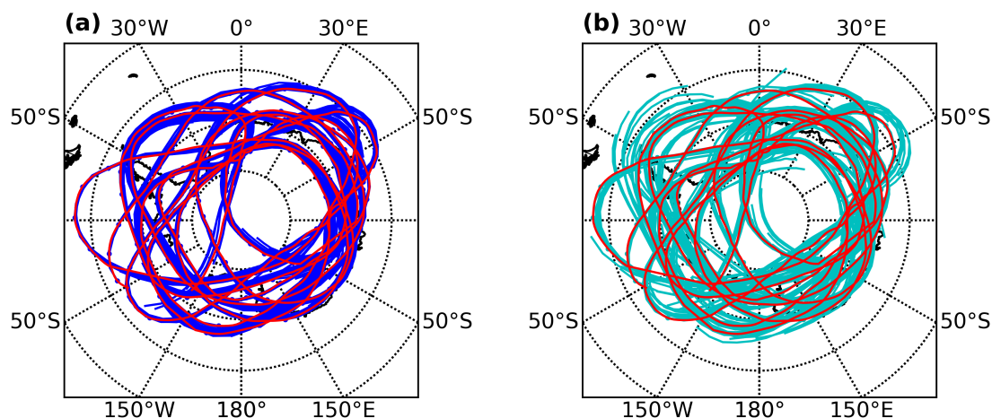
Figure 1. Trajectory of Concordiasi balloon 14, from 16 October to 22 December 2010 (red). Also plotted are trajectories calculated with (a) OA-2010 analyses (dark blue, left panel), and (b) FC-2010 forecasts (cyan, right panel). Simulated trajectories are started every 6 h from the real balloon positions, and last each for three days.
