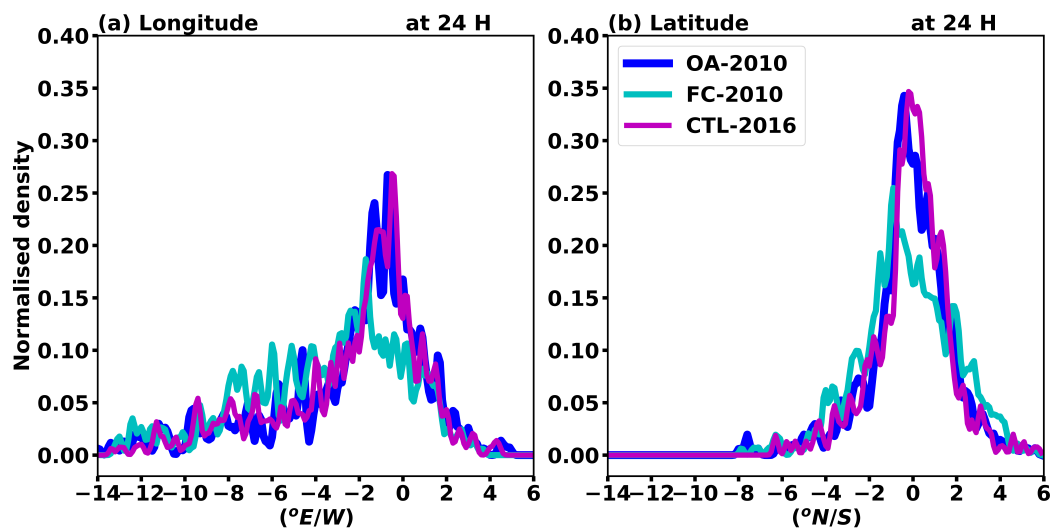
Figure 5. Probability Density Functions (PDF) of (a) longitudinal and (b) latitudinal error in the position of the simulated tropical balloons after 24 h, for trajectories calculated with winds from OA-2010 (dark blue), FC-2010 (light blue), and CTL-2016 (purple). Note that the horizontal axis covers 20^\circ , i.e., about 2200 km, and that the PDFs in longitudes are asymmetric, in contrast to those in latitudes.
