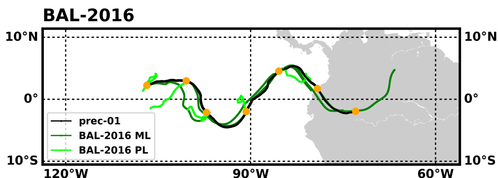
Figure 7. Same as Figure 3, but for BAL-2016 trajectories computed either on model levels (dark green) or on pressure levels (light green). The vertical resolution of the archived winds is about 10 times higher on model levels than on pressure levels (250 m vs. 2.5 km).
