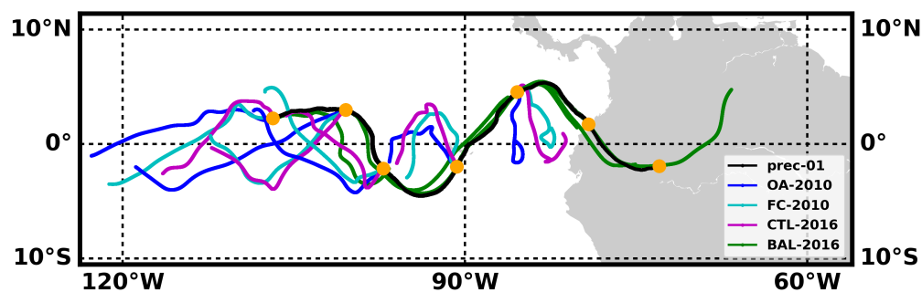
Figure 3. Pre-Concordiasi balloon 1 trajectory (black line) and those calculated with winds from OA-2010 (blue), FC-2010 (cyan), CTL-2016 (purple) and BAL-2016 (green). The period depicted starts on 31 March 2010, while the real balloon is drifting eastward toward South America. Calculated trajectories shown here start every day along the real balloon flight, and last three days. Filled orange circles are shown every 24 h on the real balloon trajectories.
