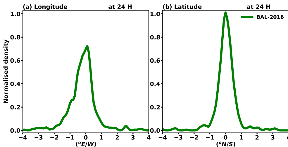
Figure 6. Same as Figure 5 but for the IFS BAL-2016 setup, in which the balloon-measured winds have been assimilated. Note the difference in the horizontal-axis range when compared with Figure 5.
