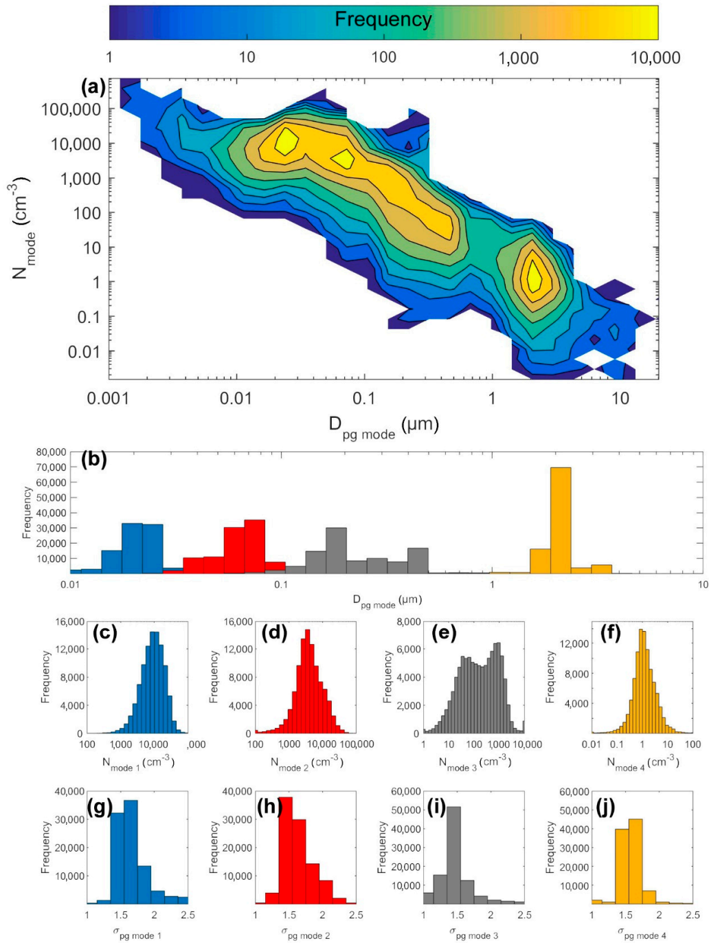
Figure 8. Modal structure of the particle number size distribution derived from the multi-lognormal fitting (5-min average). (a) Modal structure spectrum showing the dominant modes (nucleation, Aitken, accumulation, and coarse modes). Distributions of (b) mode geometric mean diameter ( D_{\text{pg}} ), (c–f) mode number concentration ( N ), and (g–j) mode geometric variance ( \sigma_{\text{pg}} ).
