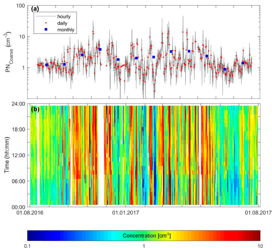
Figure 6. (a) Time series of the coarse mode (diameter 1–10 \mu m ) particle number concentration and (b) date-time spectrum showing the day-to-day and hour-to-hour variation of the number concentration; the color bar scales the number concentration ( cm^{-3} ).
