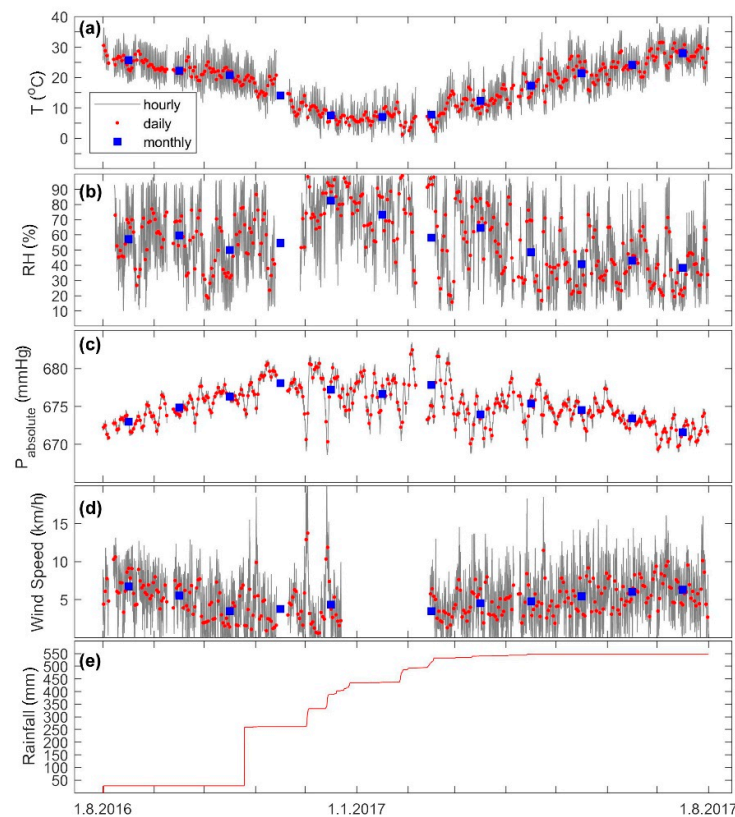
Figure 1. Time series of weather conditions during the measurement period (August 1 2016–July 31 2017) presented as hourly, daily, and monthly means for (a) ambient temperature, (b) relative humidity, (c) absolute pressure, and (d) wind speed. (e) The rainfall is presented as hourly cumulative precipitation.
