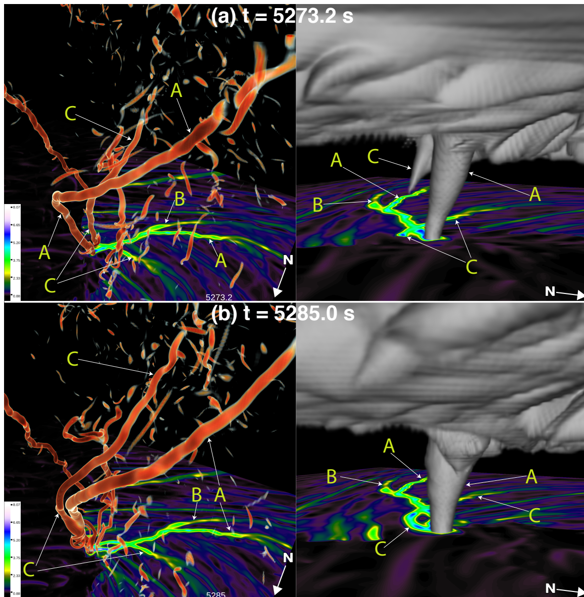
Figure 8. As in Figure 7, but at (a) t = 5273.2 \text{ s} and (b) t = 5285.0 \text{ s} . Vortex C, which has begun to wrap around vortex A, is also noted.
