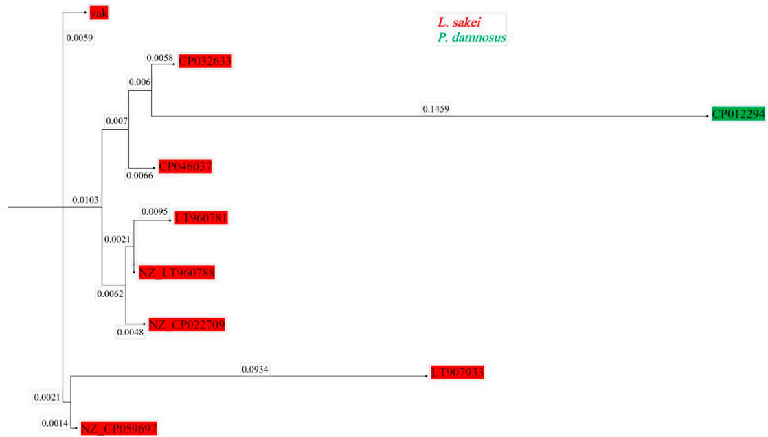
Figure S1. Phylogenetic tree of the L. sakei yak isolate and references strains. The tree was constructed using software MEGA 6.0 by the neighbor-joining method, based on whole genome sequences with 1000 replications in bootstrap testing.
