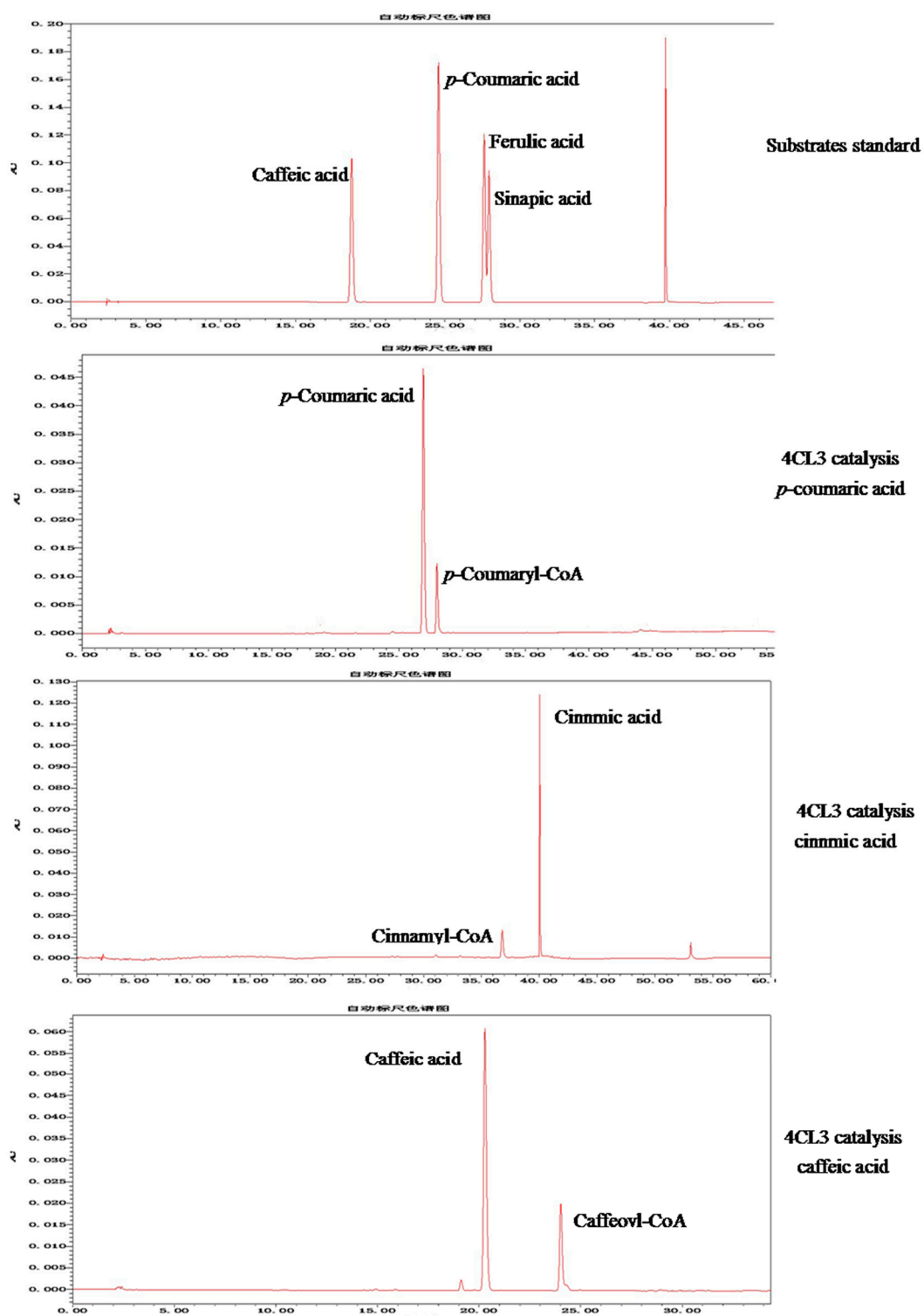
Figure S1. HPLC chromatogram of reaction products generated from the recombinant 4CL3 protein catalysis of different substrates.
