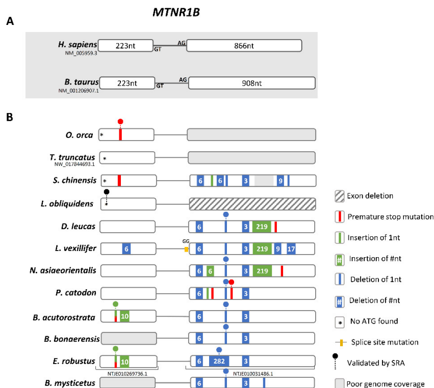
Figure 5. Mtnr1b gene annotation. (A) Schematic representation of the gene structure of human and B. taurus Mtnr1b gene (not to scale), each box represents an exon and lines represent intronic region. (B) Schematic representation of the corresponding Mtnr1b genes identified in Cetacea and location of the identified mutations. Non-canonical splice sites are indicated above the corresponding annotation.
