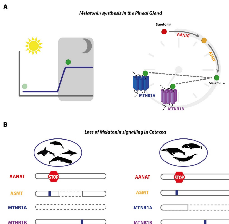
Figure 6. Melatonin synthesis and signalling modules are eroded in Cetacea. (A) Melatonin synthesis exhibits daily rhythmicity with a production peak at night (left); AANAT and ASMT sequentially convert serotonin into melatonin, which serves as ligand to two high affinity G-protein couple receptors, MTNR1A and MTNR1B (right). (B) Analysed genes from toothed whales (Odontoceti, left) and baleen whales (Mysticeti, right), premature stops, alternative splicing, indels (blue box), and complete gene erosion (dashed line), are depicted.
