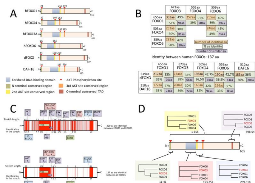
Figure 2. (A) Schematic representation of the four human FOXO members and their most important shared features; (B) identity in terms of amino acid number and percentage (related to each protein in the comparison) and number of similar amino acids. FOXOs are compared one to one (EMBOSS Needle, Matrix: EBLOSUM62, GAP penalty: 10.0, Extend penalty: 0.5 [33]). (C) Sequences that are identical in the two most similar proteins, FOXO1 and FOXO3 (top), and in all four human FOXOs (bottom) are depicted in red. (D) Phylogeny tree obtained with Clustal Omega when the indicated segments of the four human FOXO proteins are compared (the range of amino acid indicated below the boxes is relative to FOXO3 sequence).
