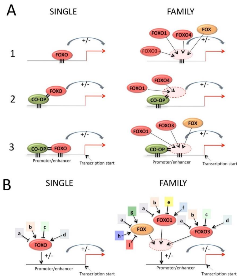
Figure 5. (A) Left side: simplified view of the major different modes of action of FOXOs: 1. Direct DNA-contact, 2. Indirect binding, through another protein making DNA-contact, 3. Pairwise binding, with both proteins making DNA-contact. Right side: Family effect for the different mode of action. (B) Left side: different pathways can influence activity of FOXOs whatever mode of action it uses. Right side: possible family effects that greatly enhance the possibilities of regulation. All the examples are arbitrary and do not reflect real situations.
