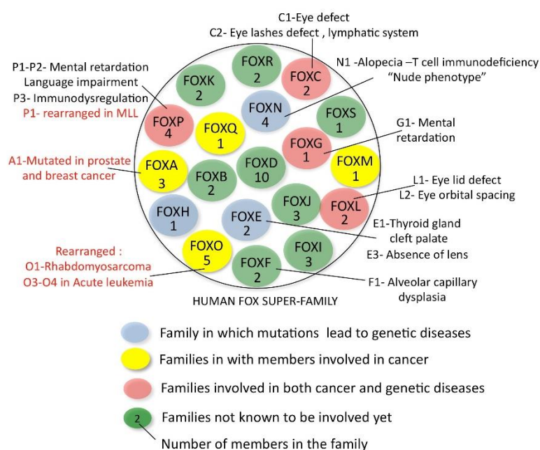
Figure 1. A schematic representation of the human FOX family of transcription factors. The members involved in genetic diseases and cancer are indicated. The arrangement of the families is independent from functional or evolution considerations.
