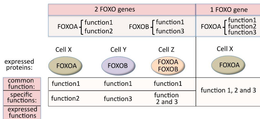
Figure 4. Possibility to express common functions in all cell types and specific functions in diverse cell types (left side) that would not be possible with the existence of a single FOXO gene (right side).
