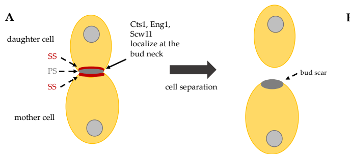
Figure 5. (A) Schematic representation of cell separation: after primary septum (PS) and secondary septa (SS) formation, Cts1, Eng1 and Scw11 activity at the daughter bud neck allows for cell separation. (B) Budding yeast exponentially growing cells stained with Calcofluor White. On the surface of mother cells these are several scars, chitin-containing rings (arrows), originated during cell division. New born daughter cells do not show bud scars.
