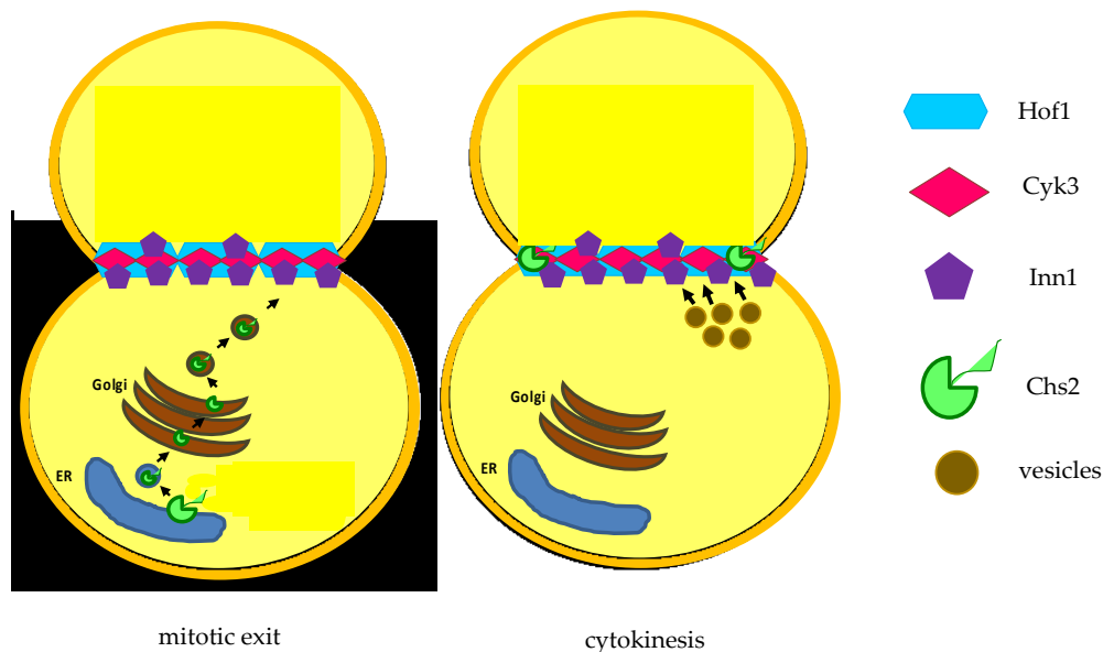
Figure 4. After mitotic exit, the chitin synthase Chs2 is translocated from endoplasmic reticulum (ER).
