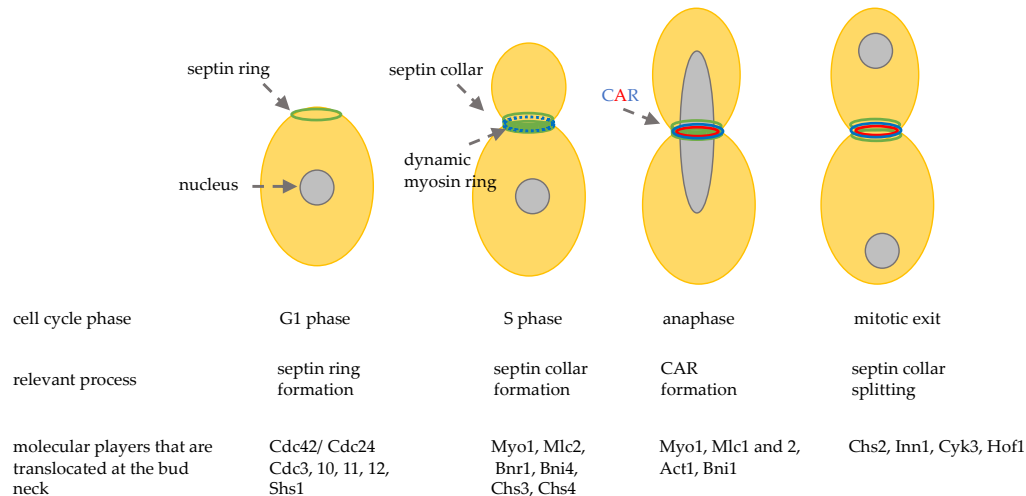
Figure 2. Schematic representation of the sequential localization at the division site of important cytokinesis players. CAR: contractile actomyosin ring.
