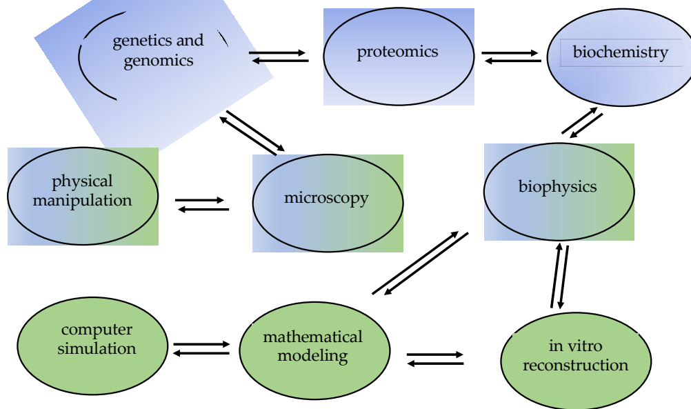
Figure 6. Several complementary methods can be used to identify cytokinesis proteins and to clarify cytokinesis mechanisms.
