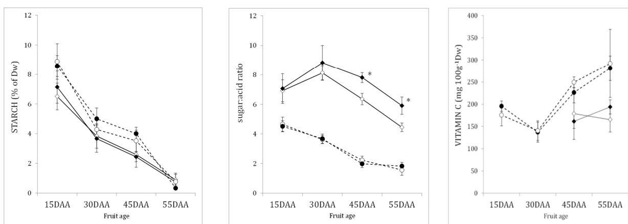
Figure 3. (a) Fructose and glucose contents, (b) citric acid and malic acid contents, (c) starch content, (d) sugar:acid ratio and (e) vitamin C content in pericarp and locular gel during the ripening of tomato fruits of R1 according to nitrogen supply N+ and N-. Fructose, glucose, citric acid and malic acid contents are expressed in g 100g -1 of dry weight. Starch content is expressed in % of dry weight. Sugar:acid ratio has no unit. Vitamin C (reduced + oxidized forms) is expressed in mg 100g -1 of dry weight. Pericarp material is presented in squares with dark lines, locular gel in circles with dotted lines. Black symbol represents N-, white symbol represents N+. Errors bars represent the standard
