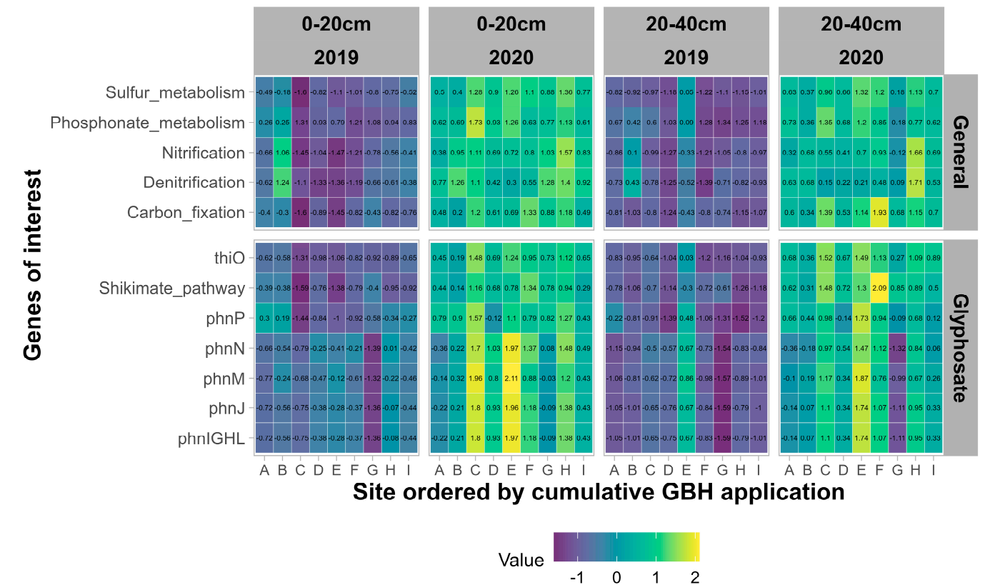
Figure 7. Normalized functional potential of prokaryotic communities for genes related to general metabolism (top) and genes related to glyphosate metabolism (bottom) for both years (2019 and 2020) and both soil horizons (0–20 cm and 20–40 cm).
