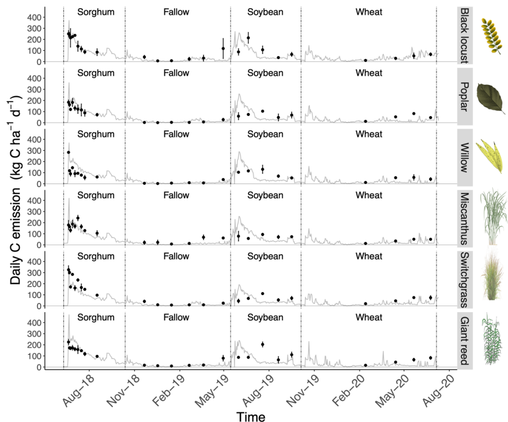
Figure 1. Results of the 2-year (2018–2020) ECOSSE simulation of C emission from soil (measured as CO 2 ) after the reversion of six different perennial energy crops to annual crops. The gray line represents modeled C emission, while the black dots represent measured values. Mean measured C emissions with error bars indicate 95% confidence intervals.
