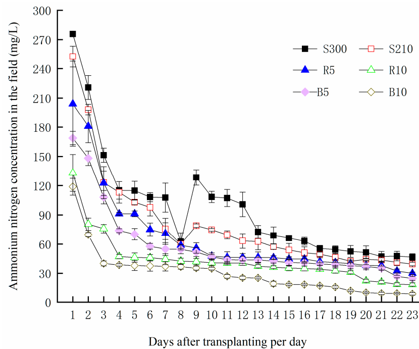
Figure 6. Daily variation of ammonium nitrogen concentration in surface water under different fertilization treatments.
