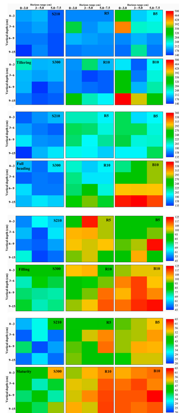
Figure 3. \text{NH}_4^+\text{-N} content in different soil layers at tillering stage, full heading stage, filling stage and maturity stage (mg/kg).
