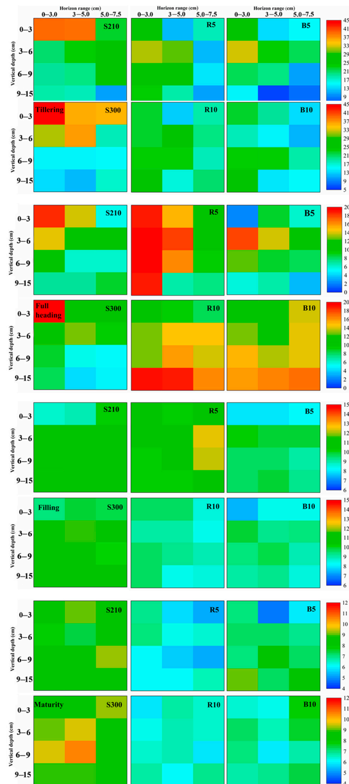
Figure 4. \text{NO}_3^- -N content in different soil layers at tillering stage, full heading stage, filling stage and maturity stage (mg/kg).
