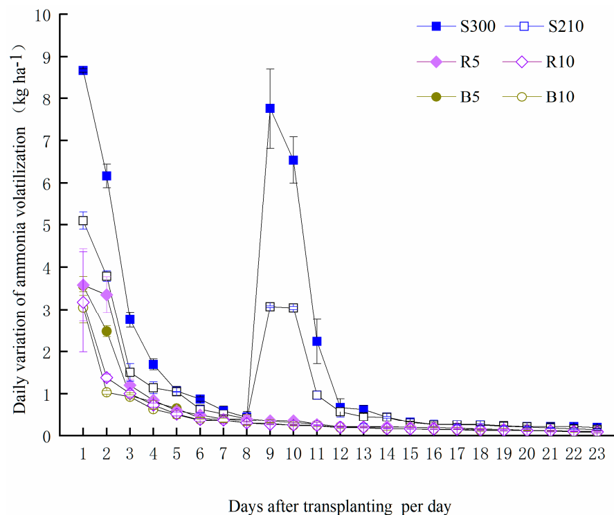
Figure 5. Daily variation of ammonia volatilization in different fertilization treatments.
