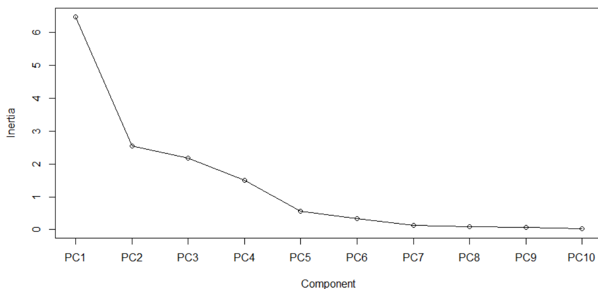
Figure A12. Scree plot from PCA analyses.
