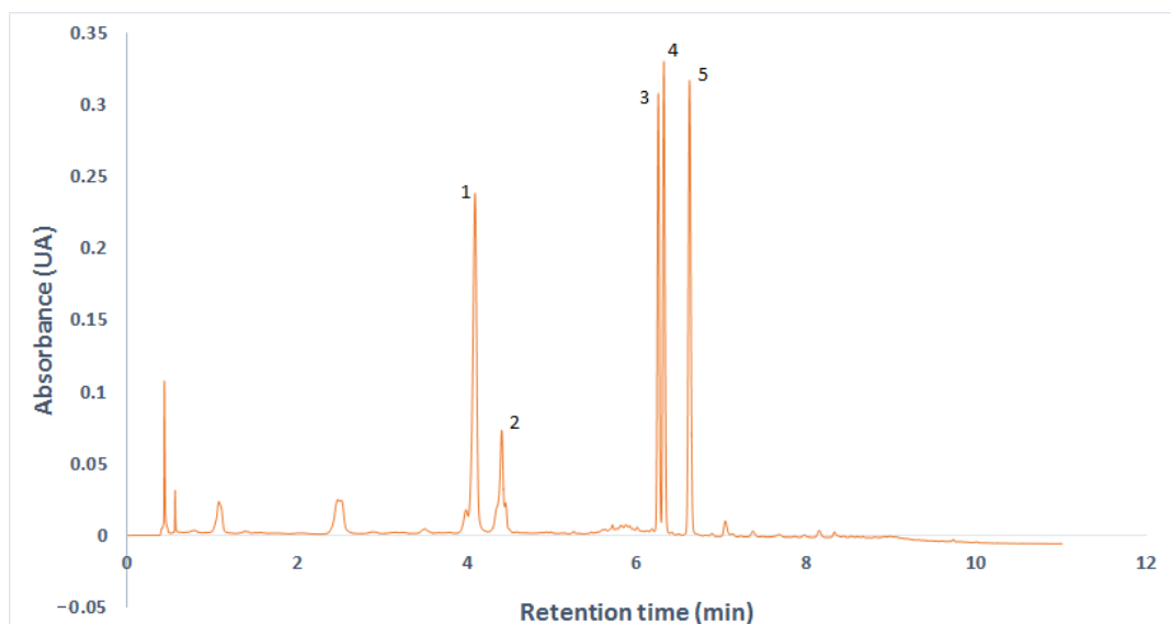
Figure 2. Chromatogram of the Covington variety (320 nm). (1) 5- O -caffeoylquinic acid (5-CQA or neochlorogenic acid), (2) 4- O -caffeoylquinic acid (4-CQA or crytochlorogenic acid), (3) 3,4-dicaffeoylquinic acid (3,4-di-CQA or isochlorogenic acid B), (4) 3,5-dicaffeoylquinic acid (3,5-di-CQA or isochlorogenic acid A), (5) 4,5-dicaffeoylquinic acid (4,5-di-CQA or isochlorogenic acid C).
