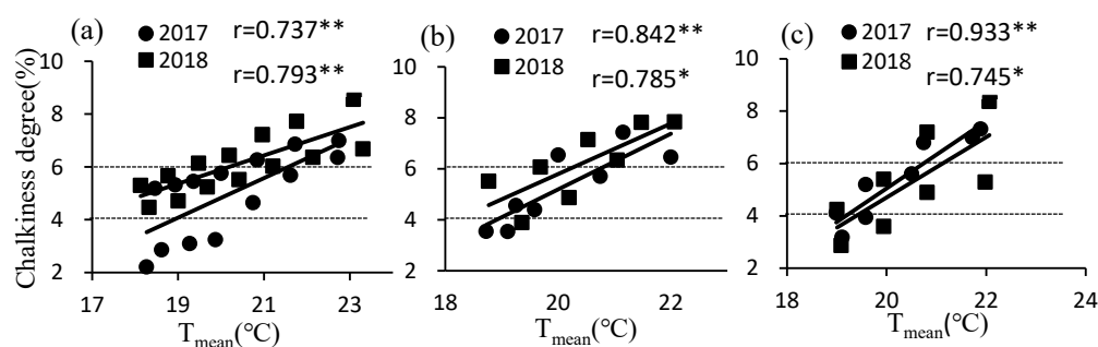
Figure 6. The correlation between chalkiness degree and the T_{mean} of rice at stage of heading-maturity (a): SMR, n = 14 , (b): SLR n = 8 , (c): LR, n = 8 , the immature treatment including T5, T6 and T7 was removed from SLR and LR). * and ** indicate p < 0.05 and p < 0.01 , respectively.
