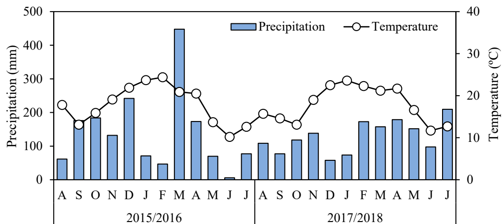
Figure S1. Monthly cumulative precipitation and average temperature (from August 2015 to July 2016 and from August 2017 to July 2018) in Cristal County/RS State, site of the experimental area of integrated crop-livestock system in southern Brazil. Source: National meteorological institute, Brazil.
