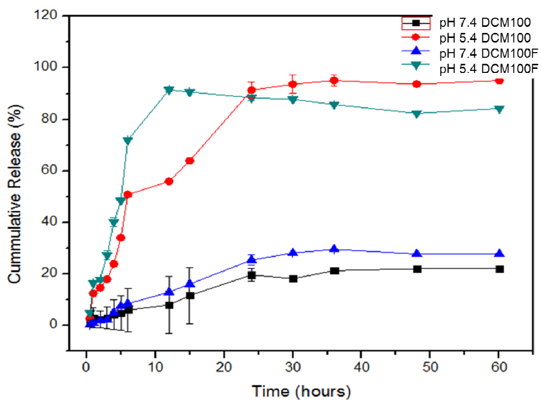
Figure S1. The release profile of DOX-loaded star-shaped FOL-PEG-PCL micelle at pH 5.4 and 7.
