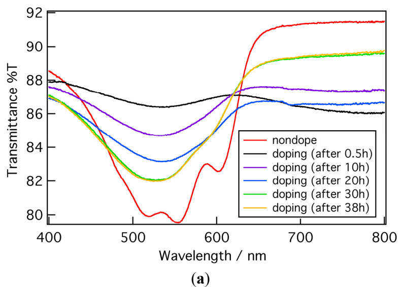
Figure S1. Time dependence of the transmittance spectra of (a) nanofiber mat and (b) P3HT/PMMA nanofiber composite film before and after doping by \text{FeCl}_3 ; measurements were carried out in air at room temperature.
