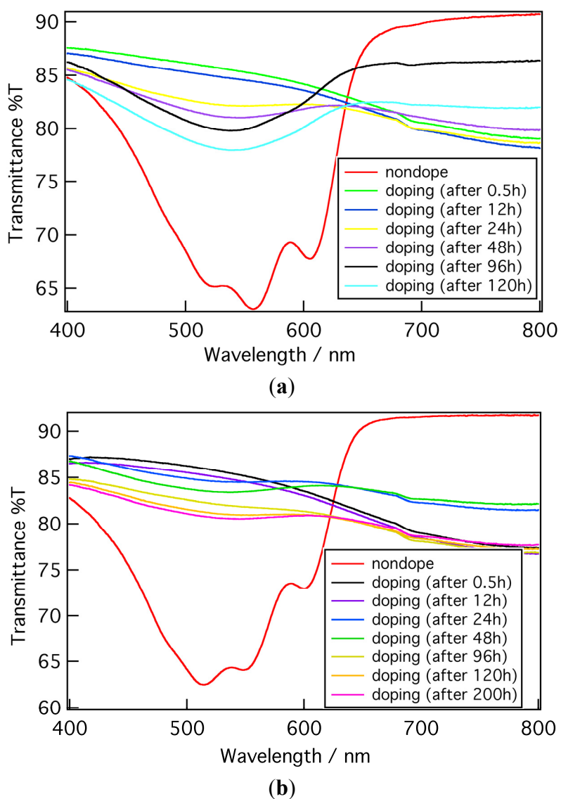
Figure S2. Time dependence of the transmittance spectra of (a) nanofiber mat and (b) P3HT/PMMA nanofiber composite film before and after doping by \text{AuCl}_3 ; measurements were carried out in air at room temperature.
