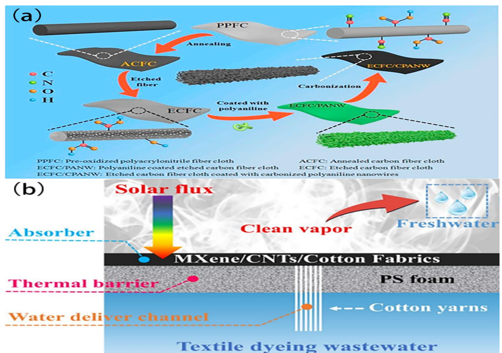
Figure 9. (a) The preparation of ECFC/CPANW SSG device. Reproduced from ref. [86], copyright 2019, Elsevier. (b) MXene/CNTs/cotton fabric ISSG device. Reproduced from ref. [58], copyright 2020, Elsevier.
