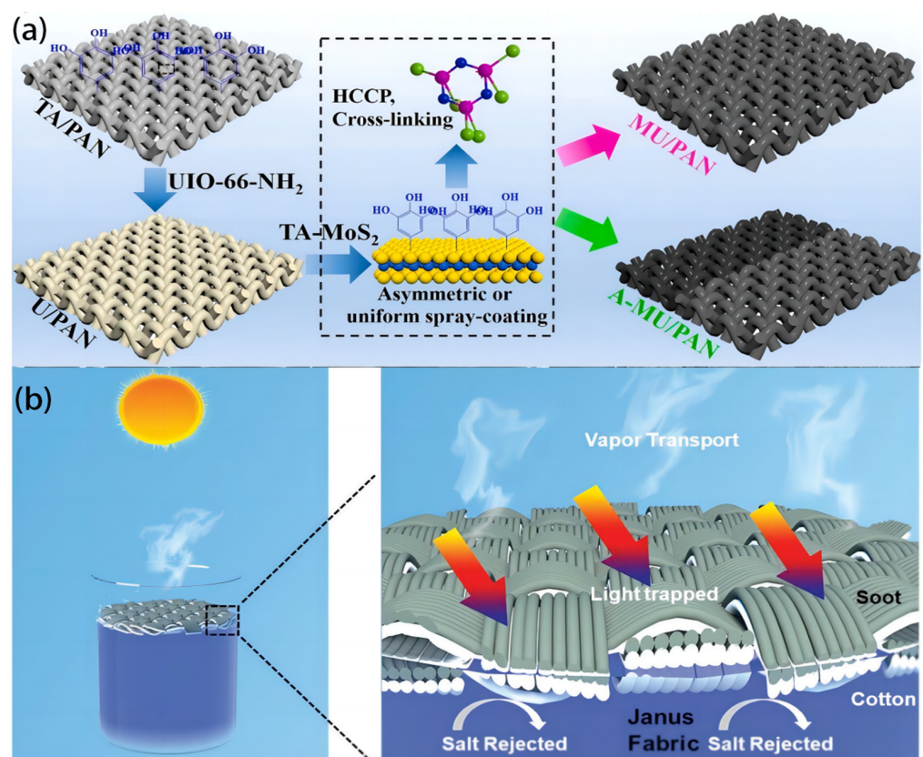
Figure 8. (a) Fabrication process of MU/PAN fabric. Reproduced from ref. [83], copyright 2021, Elsevier. (b) Design of the soot-deposited Janus fabric floating on the water surface. Reproduced from ref. [84], copyright 2019, WILEY.
