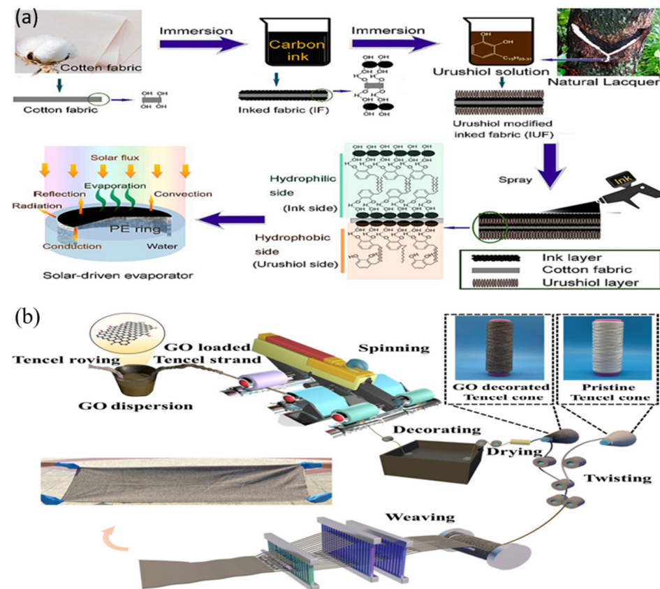
Figure 11. (a) Fabrication of the Janus ink/urushiol fabric's energy balance for the SSG device. Reproduced from ref. [89], copyright 2023, Elsevier. (b) The fabrication process of GOT fabric. Reproduced from ref. [90], copyright 2023, Springer Nature B.V.
