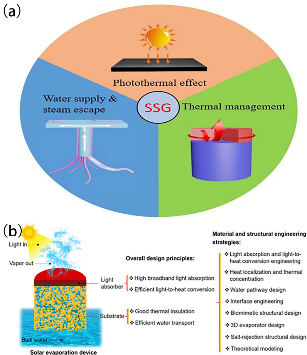
Figure 1. (a) Three main factors for ISSG design. Reproduced from ref. [61], copyright 2019, The Royal Society of Chemistry. (b) The overall principles and material and designing parameters of SSG system. Reproduced from ref. [46], copyright 2018, Elsevier.
