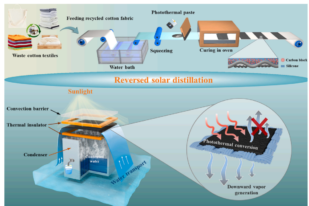
Figure 12. The process of the Janus fabric evaporator with coating process and the procedure of the Janus fabric-based ISSG. Reproduced from ref. [91], copyright 2023, Elsevier.
