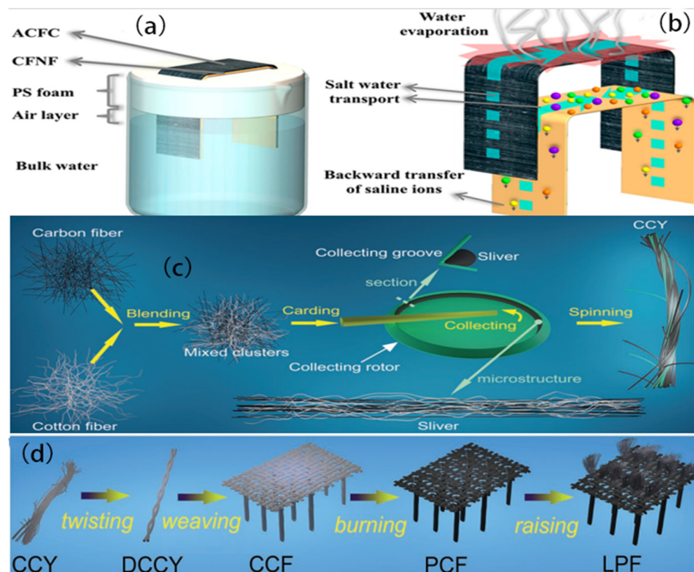
Figure 13. (a) The design of the SSG system. (b) The transportation routes of water and salt on ACFC and CFNF in ISSG. Reproduced from ref. [71], copyright 2019, American Chemical Society. (c) The blending and spinning process of carbon–cotton yarn (CCY). (d) The production process of the LPF using the CCY. Reproduced from ref. [73], copyright 2022, Wiley.
