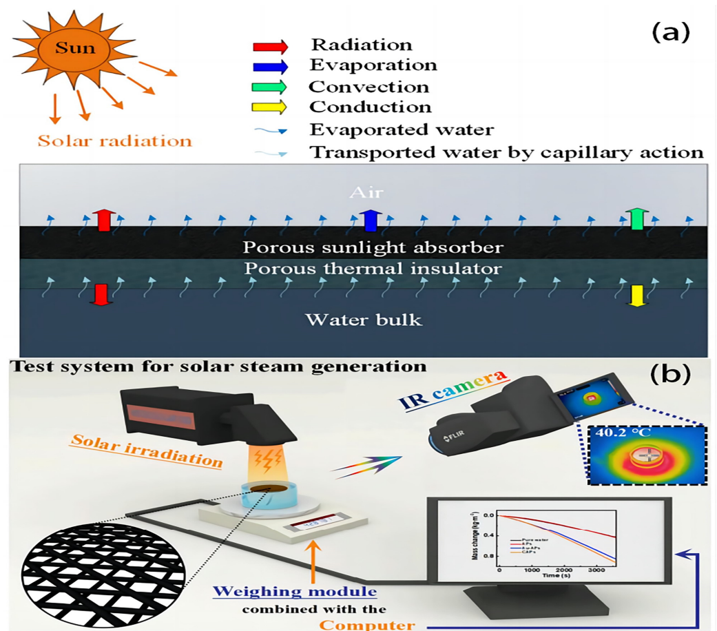
Figure 3. (a) The fundamental principles underlying the heat and mass transfer mechanisms within ISSG device. Reproduced from ref. [68], copyright 2018, Elsevier. (b) The design for assessing SSG capability. Reproduced from ref. [57], copyright 2018, Frontiers Media S.A.
