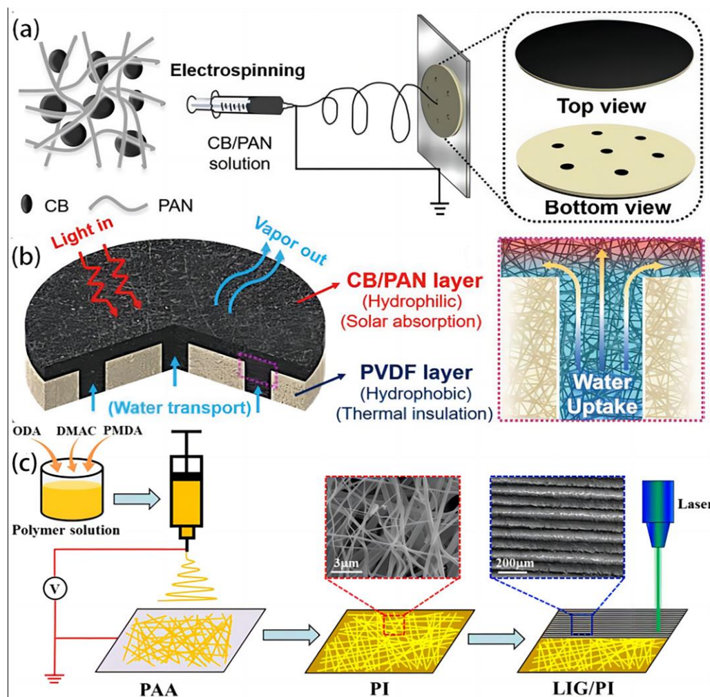
Figure 15. (a) The fabrication process and structure of the bilayer SSG device using an electrospinning method. (b) The X-section of hydrophilic CB/PAN and hydrophobic holey PVDF layers. Reproduced from ref. [97], copyright 2018, WILEY. (c) The design process of PI membrane and LIG/PI membrane. Reproduced from ref. [60], copyright 2020, American Chemical Society.
