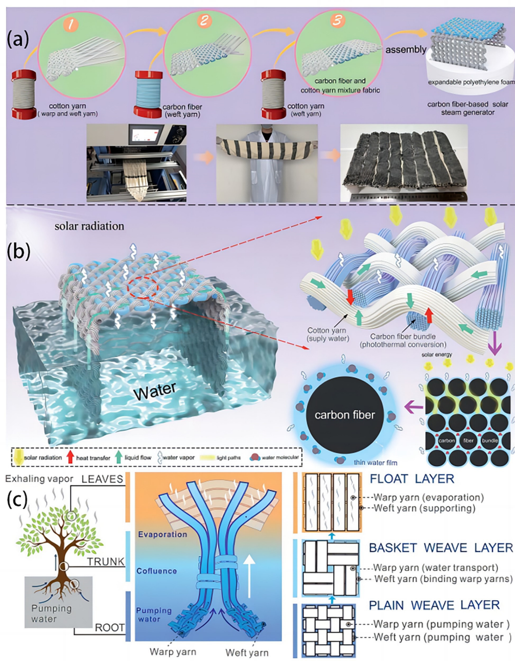
Figure 5. (a) The manufacturing of the CCMF-based ISSG including the design of CCMFs by a textile weaving technique. (b) The operation concepts of CCMF-based ISSG. Reproduced from ref. [75], copyright 2020, The Royal Society of Chemistry. (c) Schematic illustration of the tree shape and the representative biomimetic design of the TBFF. Reproduced from ref. [45], copyright 2021, The Royal Society of Chemistry.
