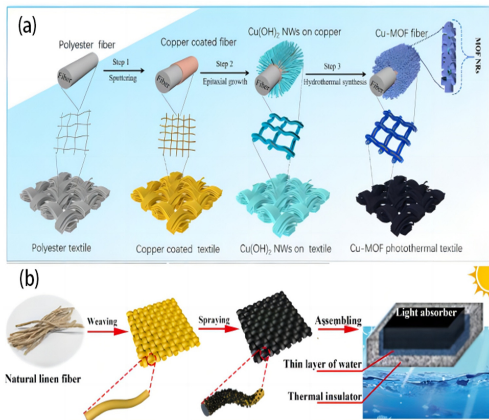
Figure 7. (a) Schematic illustration of the synthetic process for CMPT. Reproduced from ref. [82], copyright 2021, Elsevier. (b) The natural linen fiber, the original linen fabric (LF), the LF covered with candle soot (LFS), and the integrated LFSTM composed of LFS and a thermal management section (polystyrene). SEM images of original linen fiber. Reproduced from ref. [31], copyright 2020, American Chemical Society.
