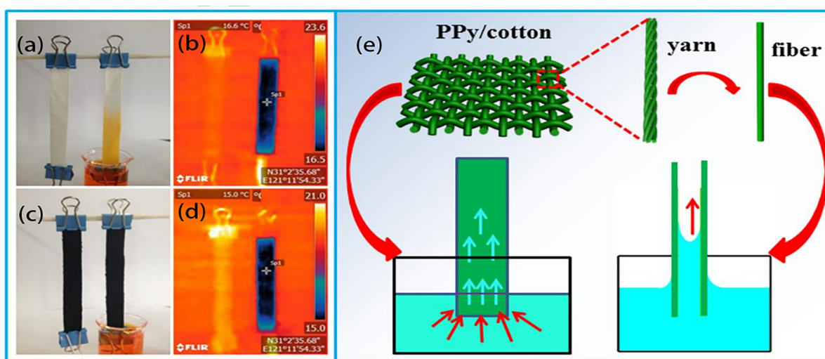
Figure 4. The optical images illustrating the vascular absorption of water by pristine cotton (a) and PPy/cotton. (c) IR photos demonstrate the temperature variations in pristine cotton (b) and PPy/cotton, (d) both before and after capillary absorption. (e) The process of capillary water absorption in PPy/cotton fabric. Reproduced from ref. [72], copyright 2018, Elsevier.
