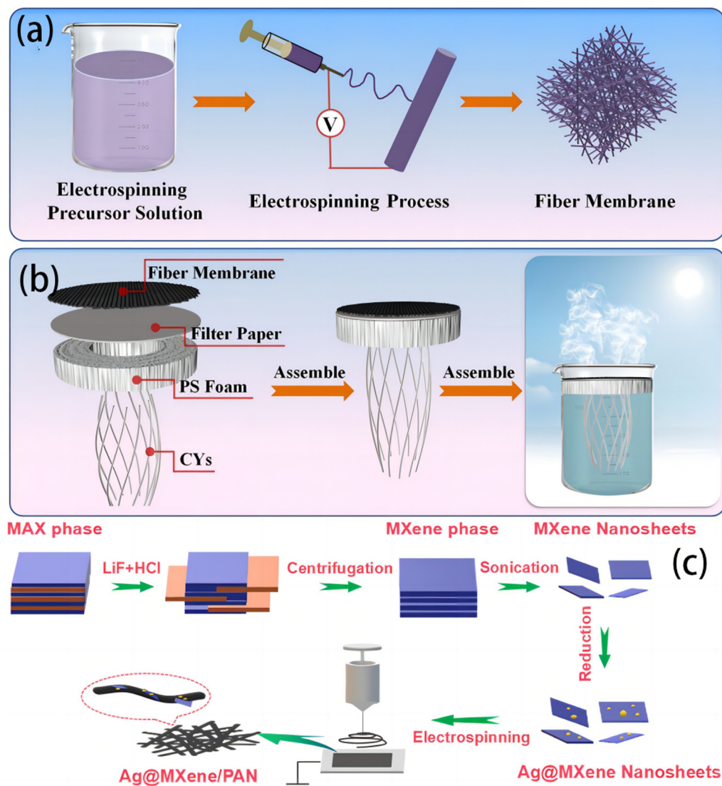
Figure 16. (a) The fabrication of (a) electrospinning fiber membranes and assembly of (b) interfacial water evaporator. Reproduced from ref. [99], copyright 2020, Elsevier. (c) The diagram of the design of Ag@MXene/PAN nanofiber membrane. Reproduced from ref. [98], copyright 2021, Elsevier.
