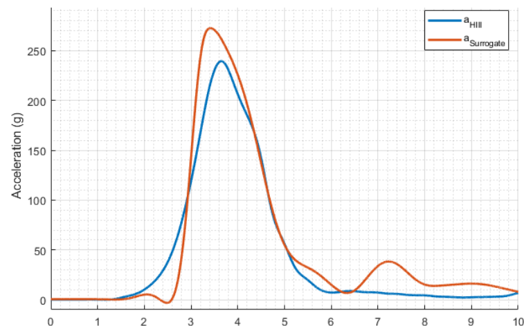
Figure 4. Calibration curves for the Hybrid III head form (blue) and the 3D-printed head surrogate (red).
