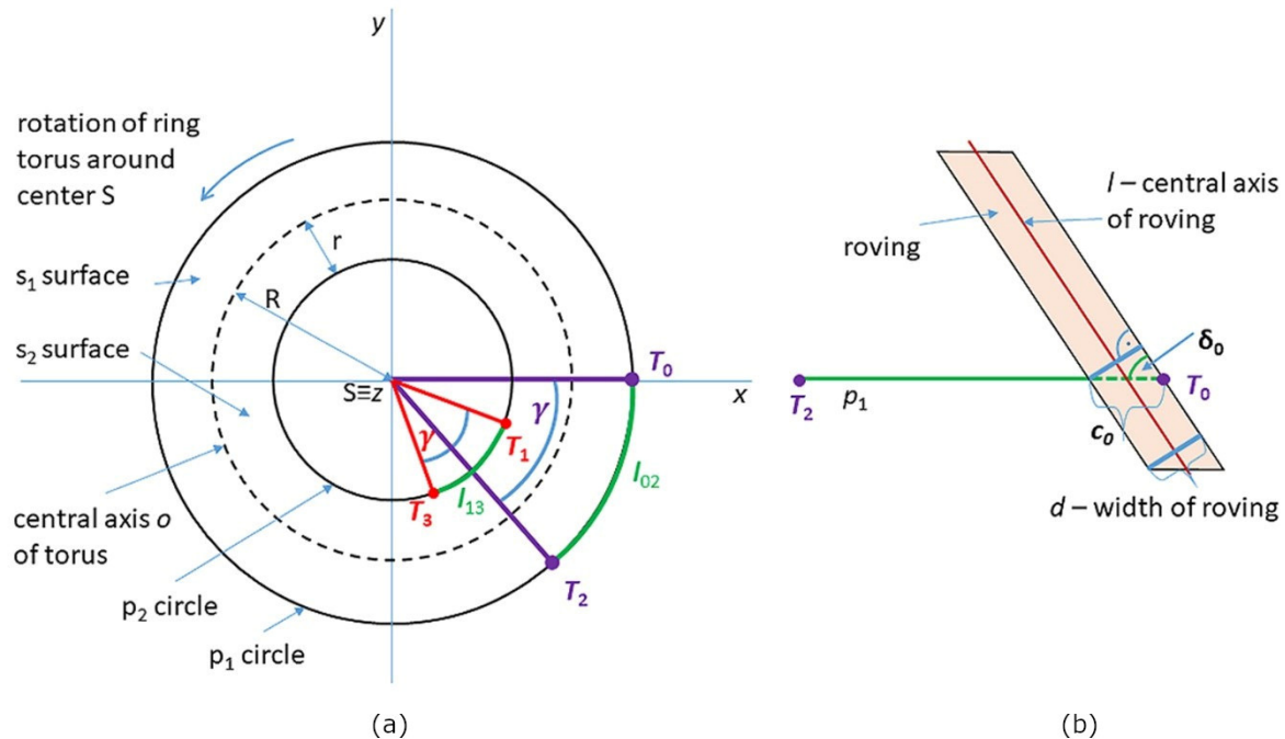
Figure 11. (a) Arc length part l_{02} of circle p_1 and arc length part l_{13} of circle p_2 . (b) Laying a roving of width d at an angle \alpha_{ext} (relation 18a/). Value c_0 indicates the length of the wound roving on connecting points T_0 and T_2 .
