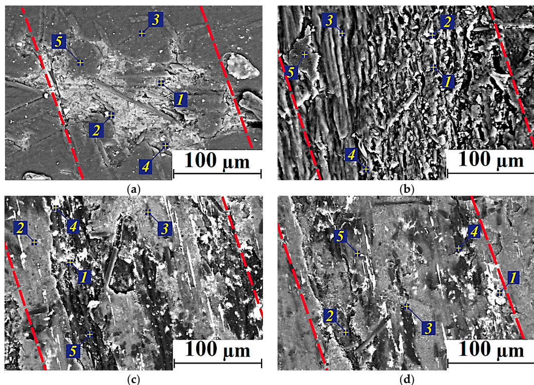
Figure 8. SEM-micrographs of the wear tracks on the PEI/10CCF/10PTFE (a), PEI/10CCF/10Gr (b), PEI/10CCF/10MoS 2 (c), PEI/10CCF/23MoS 2 (d) composites after the tribological tests at T = 180 °C (wear track edges marked with red dotted lines).
