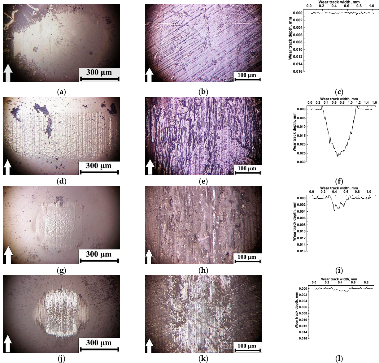
Figure 7. Optical micrographs of the friction scar surfaces on the ceramic counterpart ( T = 180 \text{ °C} ) after the tribological tests of the PEI/10CCF/10PTFE (a–c), PEI/10CCF/10Gr (d–f), PEI/10CCF/10MoS 2 (g–i), PEI/10CCF/23MoS 2 (j–l) composites.
