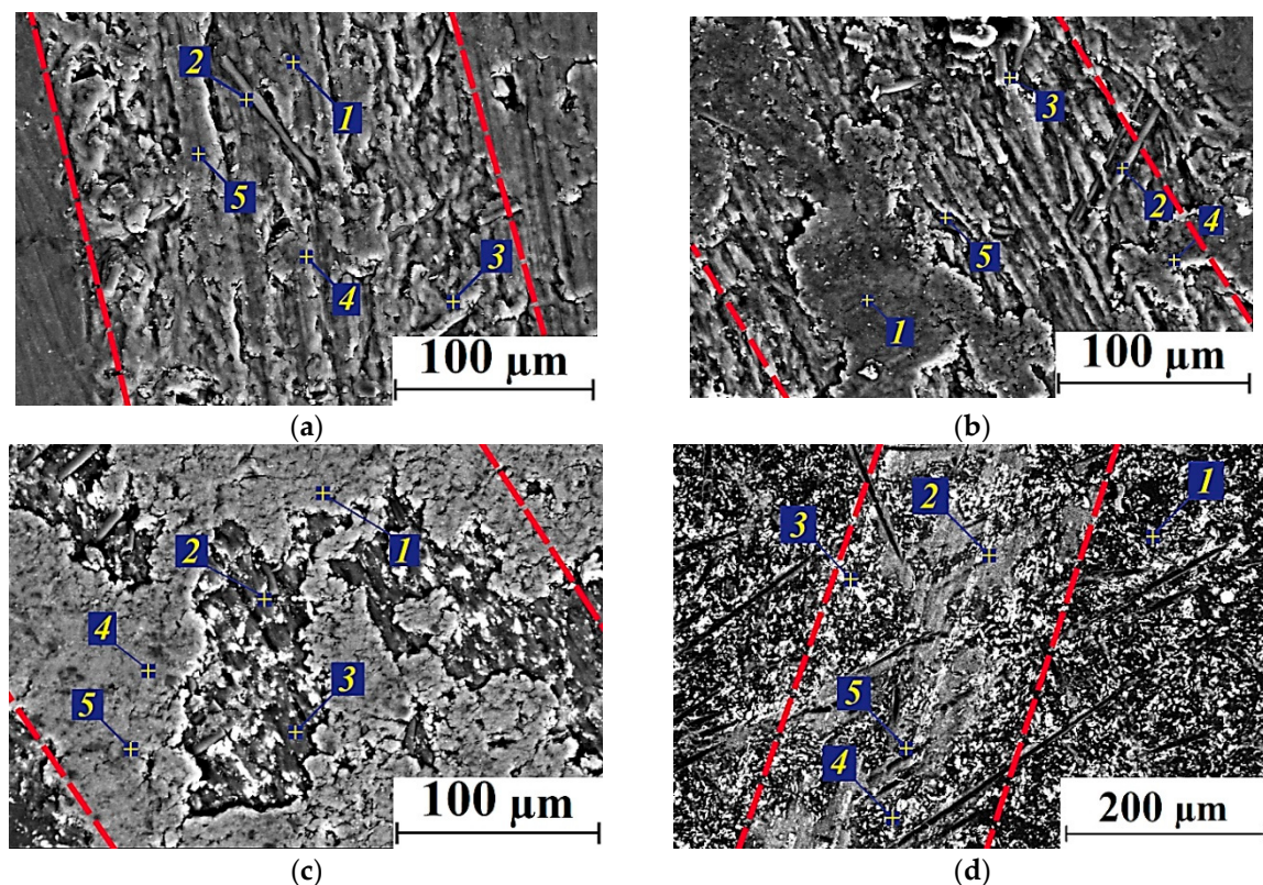
Figure 10. SEM-micrographs of the wear track surfaces on the PI/10CCF/10PTFE (a), PI/10CCF/10Gr (b), PI/10CCF/10 \text{MoS}_2 (c), PI/10CCF/23 \text{MoS}_2 (d) composites after the tests at the temperature of 180\text{ }^{\circ}\text{C} (wear track edges marked with red dotted lines).
