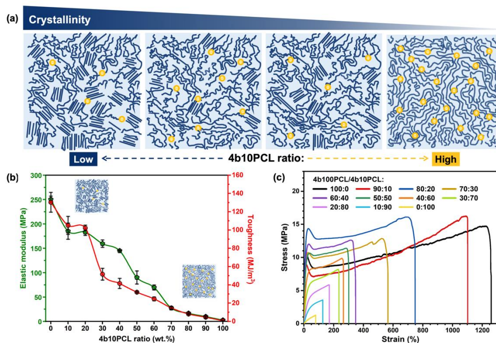
Figure 3. Crystallinity-dominant effect on the mechanical properties of 4b100PCL/4b10PCL polymer blends at 20 °C. (a) Schematic illustrations of the decreasing crystallinity of the 4b100PCL/4b10PCL polymer blends with the increase of the amorphous 4b10PCL ratio, (b) Elastic modulus and toughness, and (c) stress-strain curves of the 4b100PCL/4b10PCL polymer blends with gradient 4b10PCL ratios.
