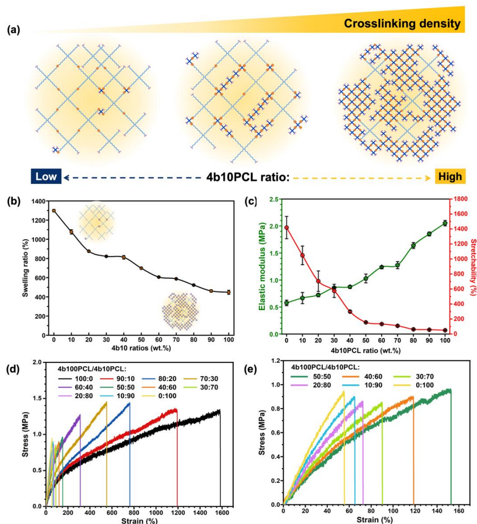
Figure 4. Crosslinking density-dominant effect on the mechanical properties of 4b100PCL/4b10PCL polymer blends at 60 °C. (a) Schematic illustrations of increasing crosslinking densities of the 4b100PCL/4b10PCL polymer blends with the increase of the short-chained 4b10PCL ratios, (b) swelling ratios measured at room temperature, (c) elastic modulus and stretchability, (d) stress-strain curves of the 4b100PCL/4b10PCL polymer blends with gradient 4b10PCL ratios, and (e) zoomed in stress-strain curves of the 4b100PCL/4b10PCL polymer blends with 0–50 wt.% of 4b10PCL ratios.
