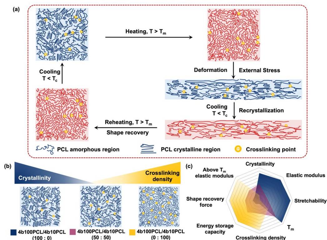
Figure 1. (a) Shape-memory mechanism for semicrystalline PCL-based SMPs. (b) Decreased crystallinity gradient and increased crosslinking density gradient achieved by the manipulation of amorphous 4b10PCL ratios in 4b100PCL/4b10PCL polymer blending systems. (c) Comparison of major physical properties and their expected correlations with crystallinity and crosslinking density in 4b100PCL/4b10PCL polymer blending systems. Different 4b100PCL/4b10PCL ratios are indicated by different colors.
