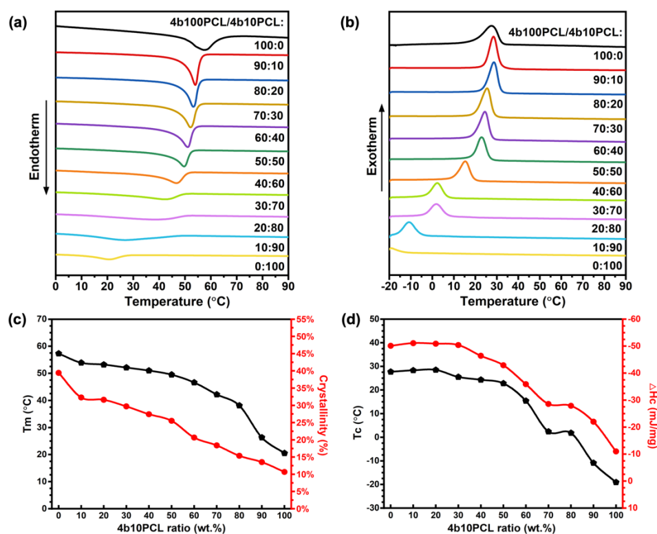
Figure 2. Thermal properties of 4b100PCL/4b10PCL polymer blends prepared with different 4b10PCL ratios. (a) DSC melting curves, (b) DSC crystallization curves, (c) melting temperature and crystallinity, and (d) crystallization temperature and \Delta H_c of the 4b100PCL/4b10PCL polymer blends.
