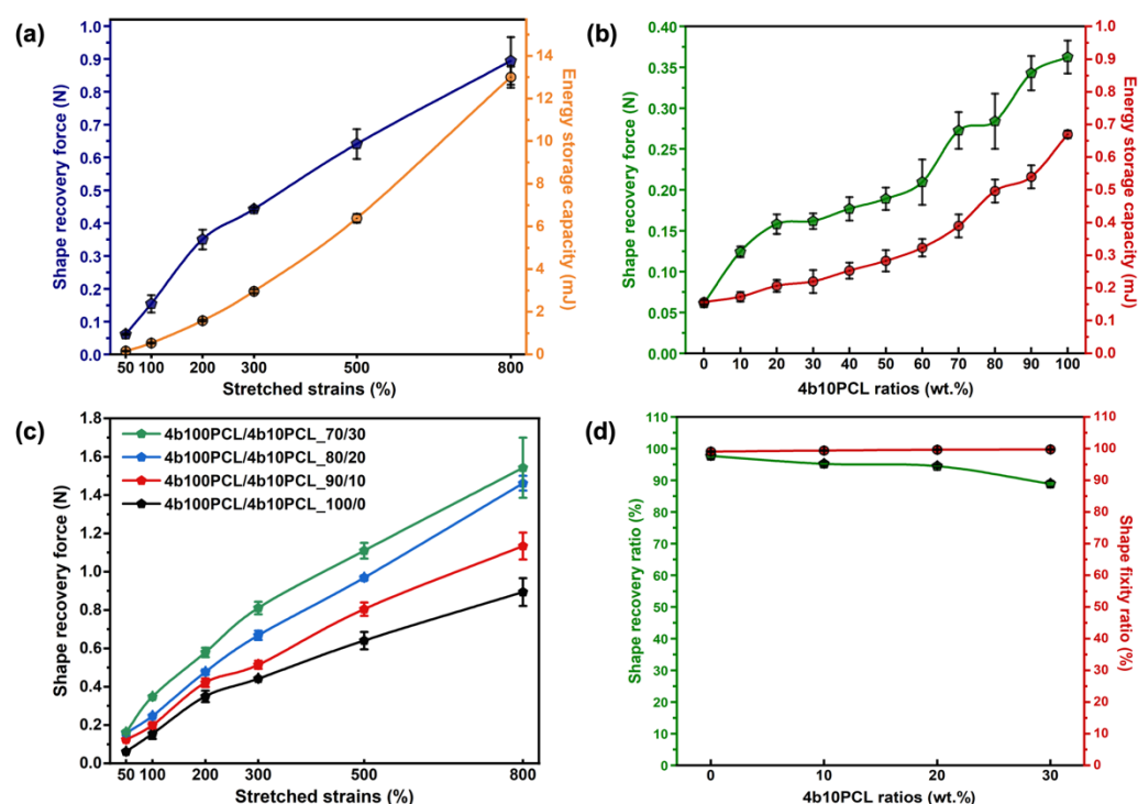
Figure 5. Shape-memory properties, shape recovery forces, and their correlations with the energy storage capacities of the 4b100PCL/4b10PCL polymer blends. Shape recovery force and energy storage capacities of (a) 4b100PCL at different stretched strains and (b) 4b100PCL/4b10PCL polymer blends with gradient 4b10PCL ratios at 50% stretched strain. (c) Shape recovery forces of 4b100PCL/4b10PCL polymer blends with 0–30 wt.% of 4b10PCL ratios at different stretched strains. (d) Shape recovery ratios and shape fixities of 4b100PCL/4b10PCL polymer blends with 0–30 wt.% of 4b10PCL ratios at a large deformation of 800%.
