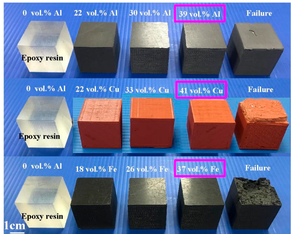
Figure 15. Experimental results of the upper limit of fillers.
