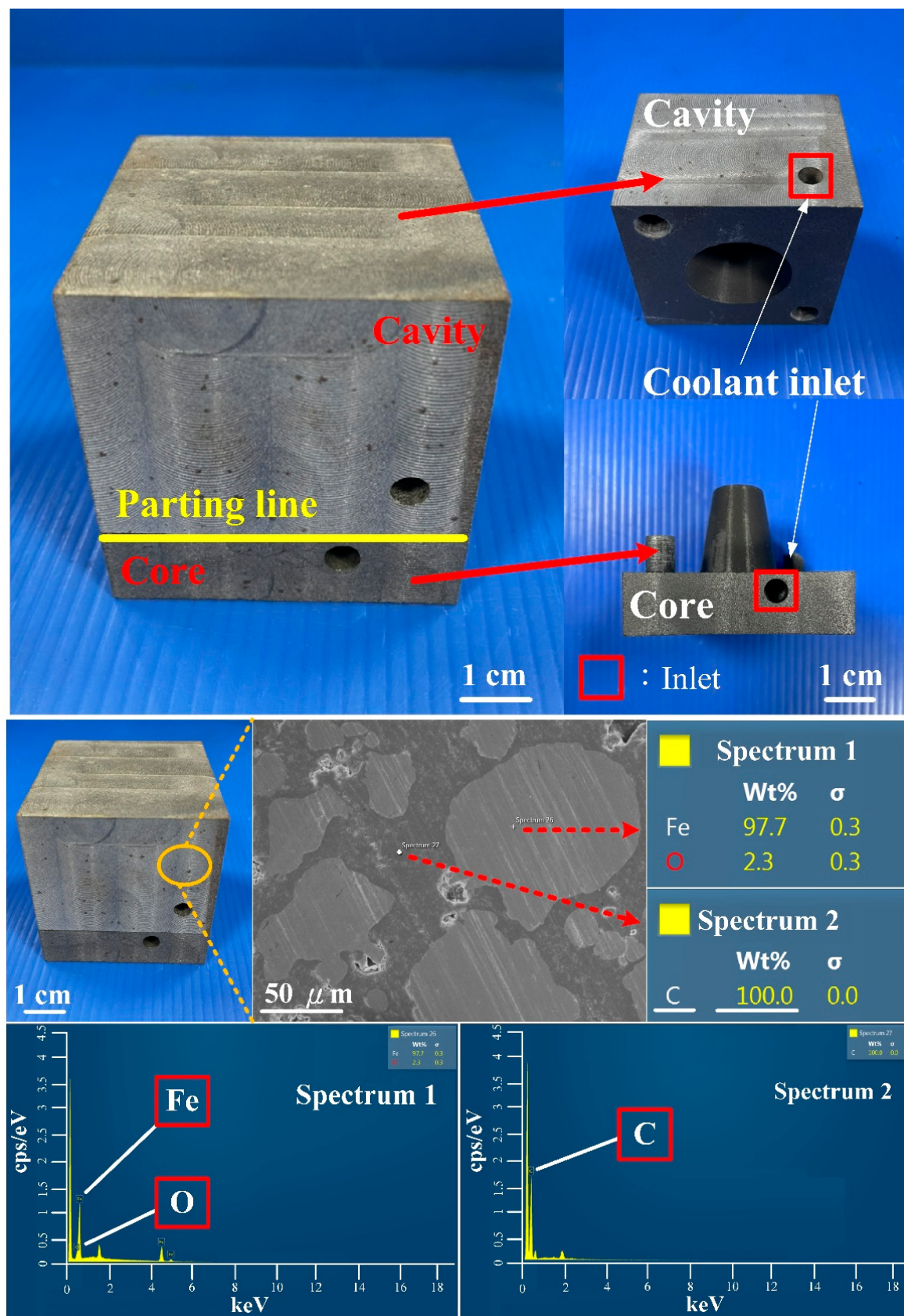
Figure 20. SEM micrographs and chemical composition of wax injection mold fabricated by epoxy resin added with 37 vol.% Fe powder.
