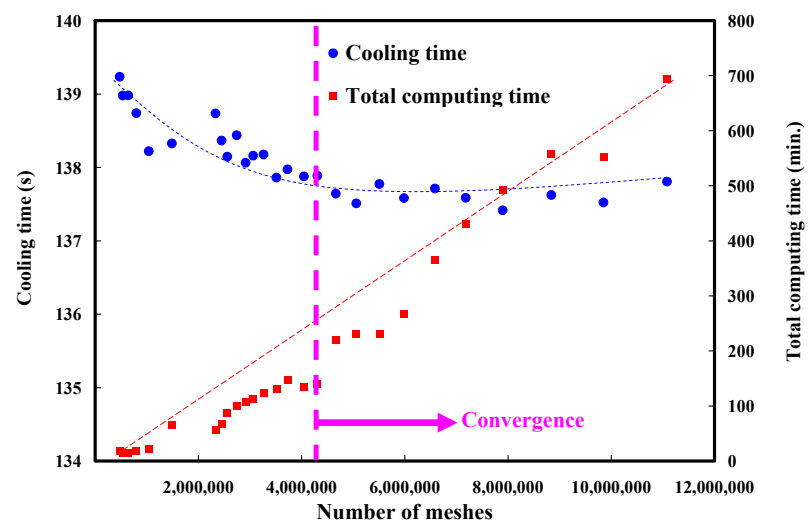
Figure 10. Number of meshes as a function of cooling time and total computing time of numerical analysis.
