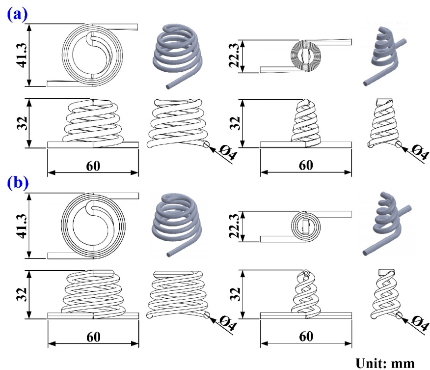
Figure 5. Layouts of (a) PCCC and (b) CCCC.
