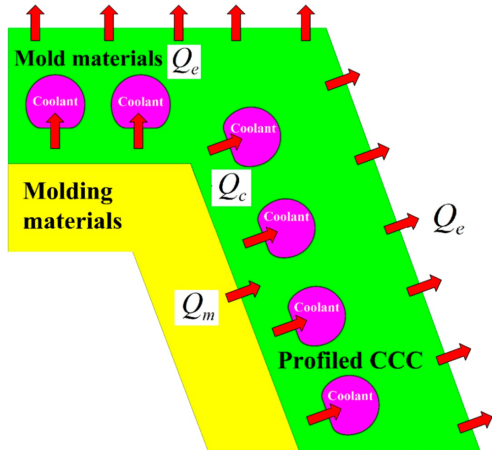
Figure 23. Schematic illustration of the heat fluxes of PCCC during the cooling stage.
