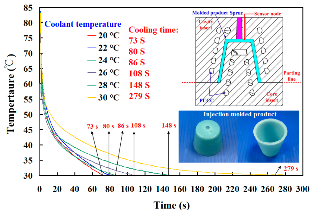
Figure 22. Cooling time of the wax pattern fabricated with epoxy resin added with 39 vol.% Al powder.
