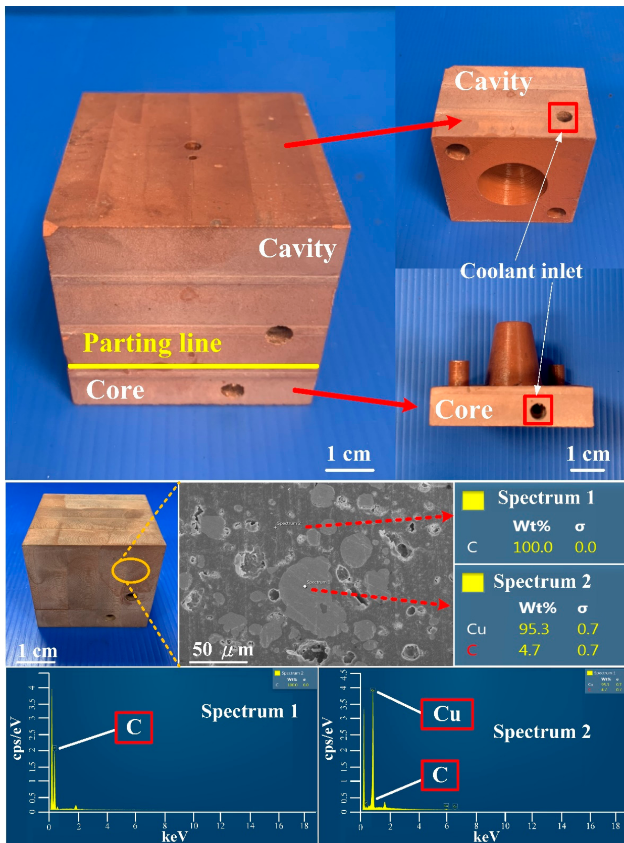
Figure 17. SEM micrographs and chemical composition of wax injection mold fabricated by epoxy resin added with 41 vol.% Cu powder.
