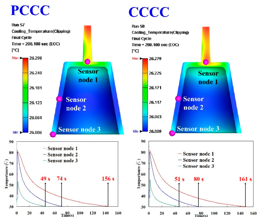
Figure 13. Simulation results of the cooling time of the injection-molded part for the injection mold fabricated by epoxy resin added with 39 vol.% Al powder.
