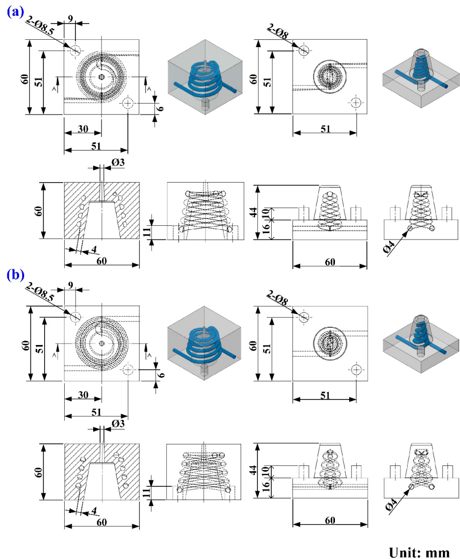
Figure 6. CAD model and dimensions of the wax injection molding tool with (a) PCCC and (b) CCCC.
