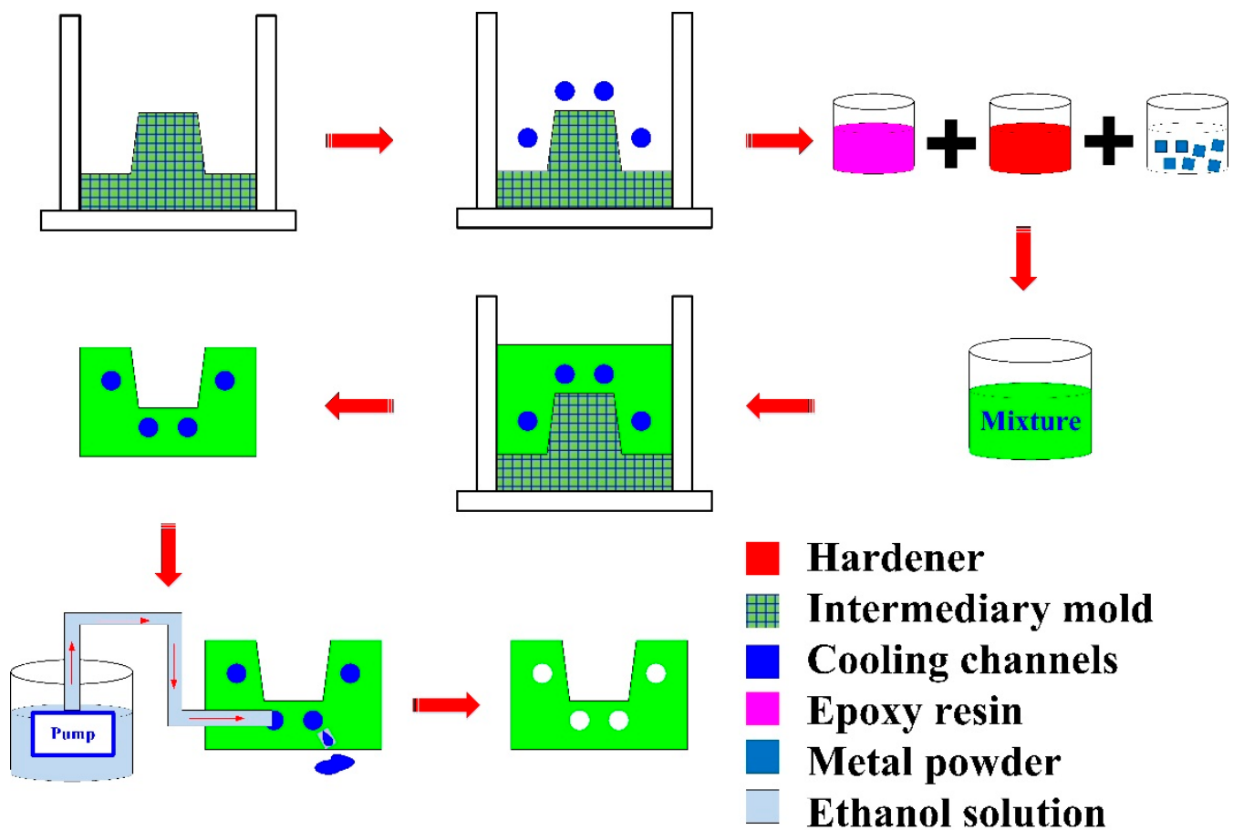
Figure 8. Schematic illustrations of the production process of the wax injection molding tool with cooling channel.
