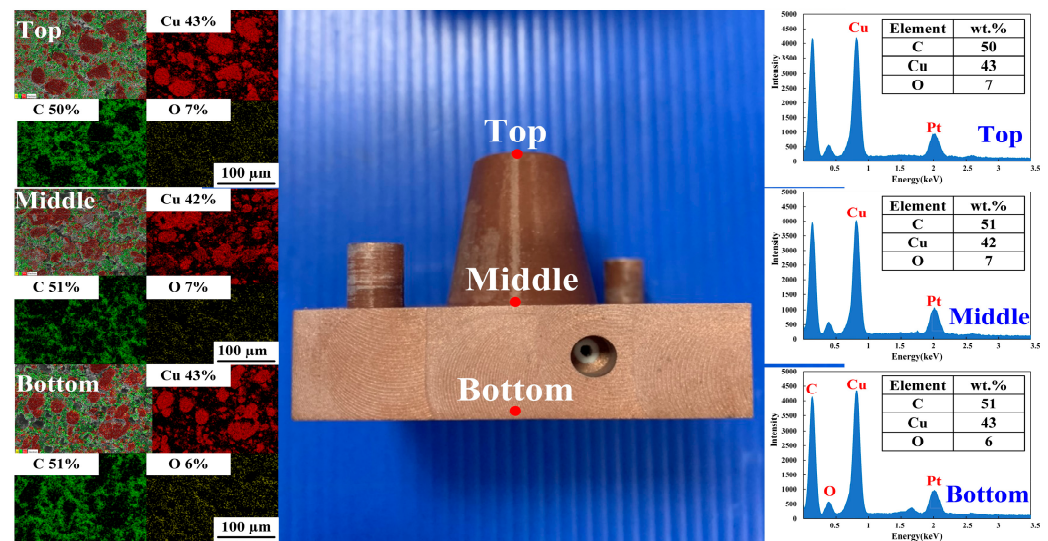
Figure 21. Precipitation analysis of the core insert fabricated by epoxy resin added with Cu powder.
