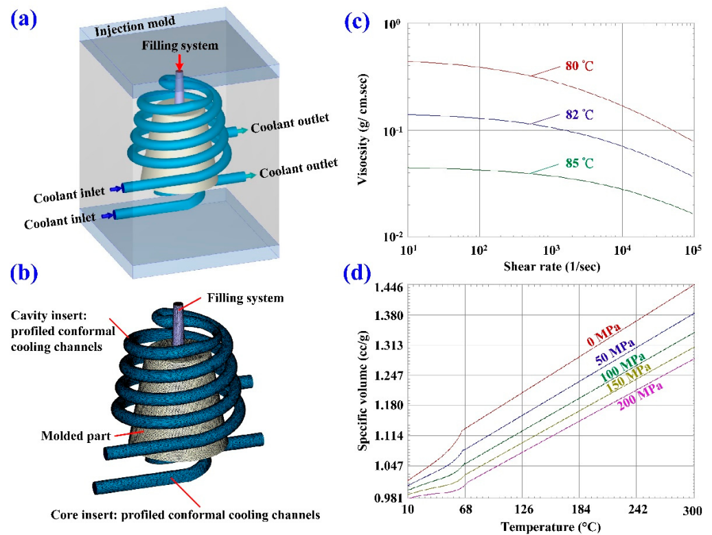
Figure 7. Details of the wax injection molding simulation conditions; (a) configuration of the simulation model, (b) finite element mesh of profiled conformal cooling channels, filling system, and injection-molded parts, (c) viscosity chart, and (d) PVT diagram of the molding materials.
