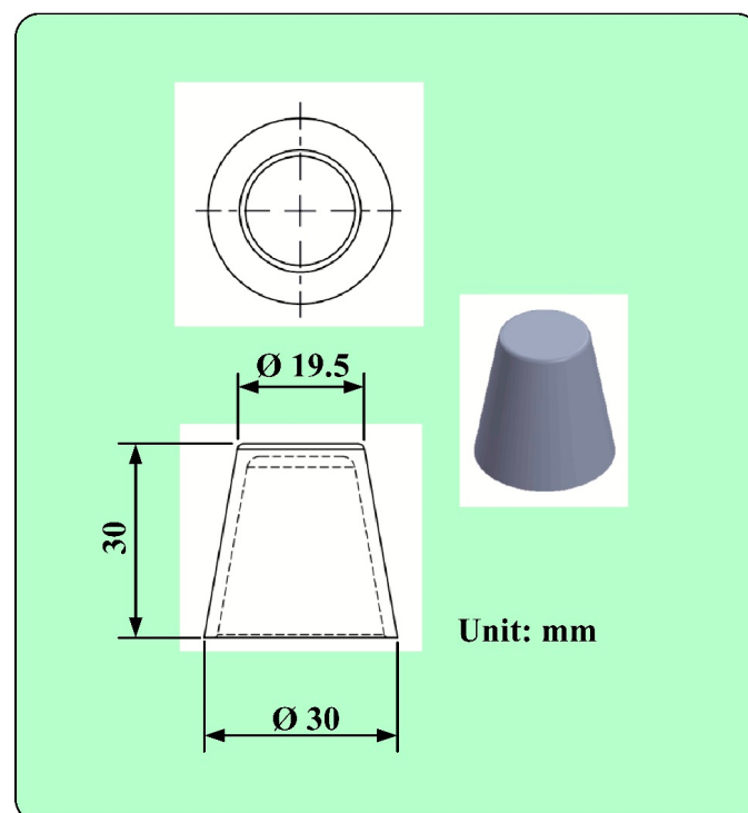
Figure 2. 3D CAD model of the wax pattern.
