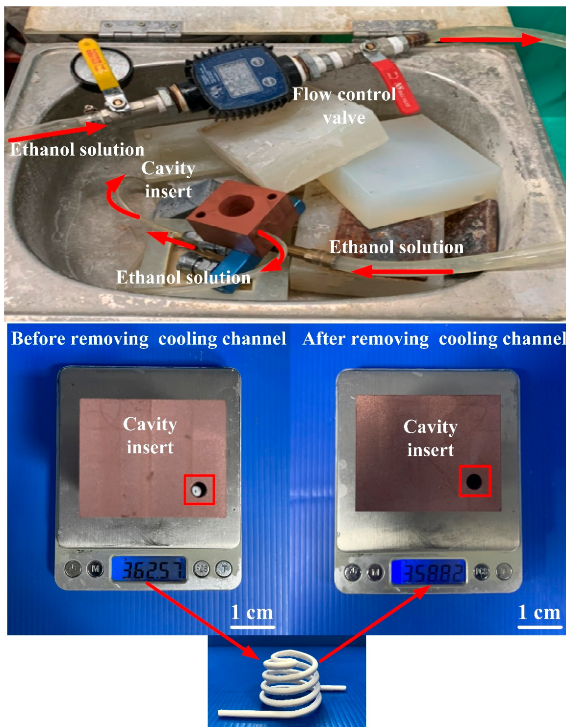
Figure 18. Wax injection mold before and after removing PCCC.
