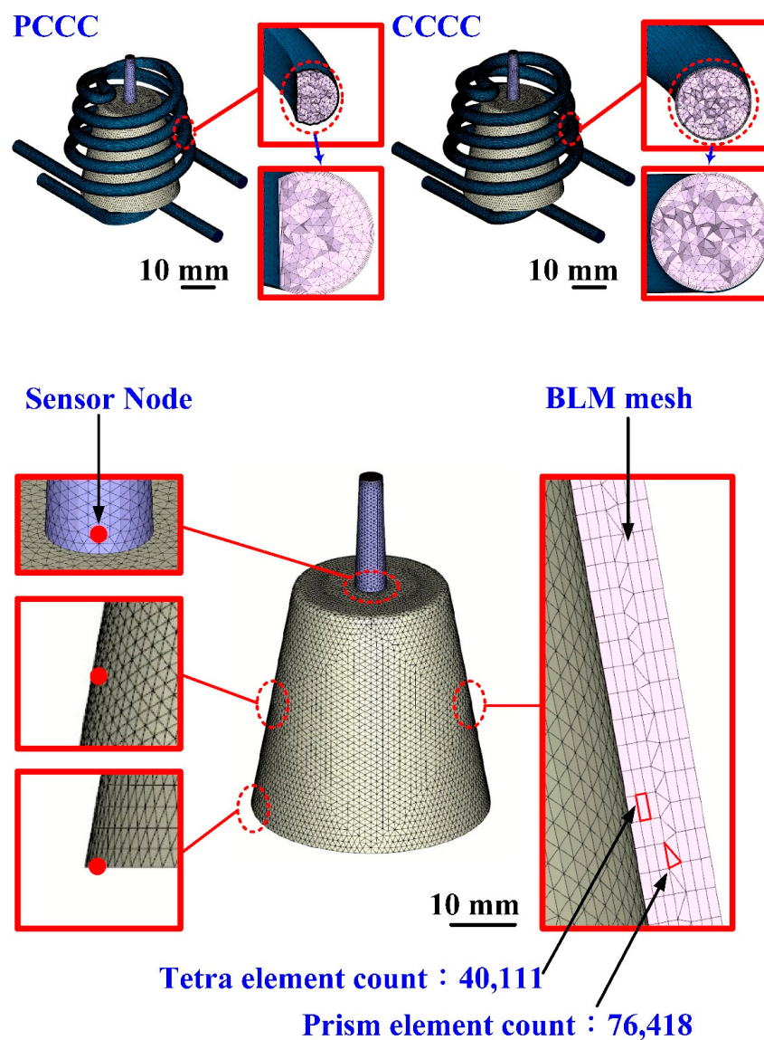
Figure 11. Mesh of the injection-molded part and cooling channels.
