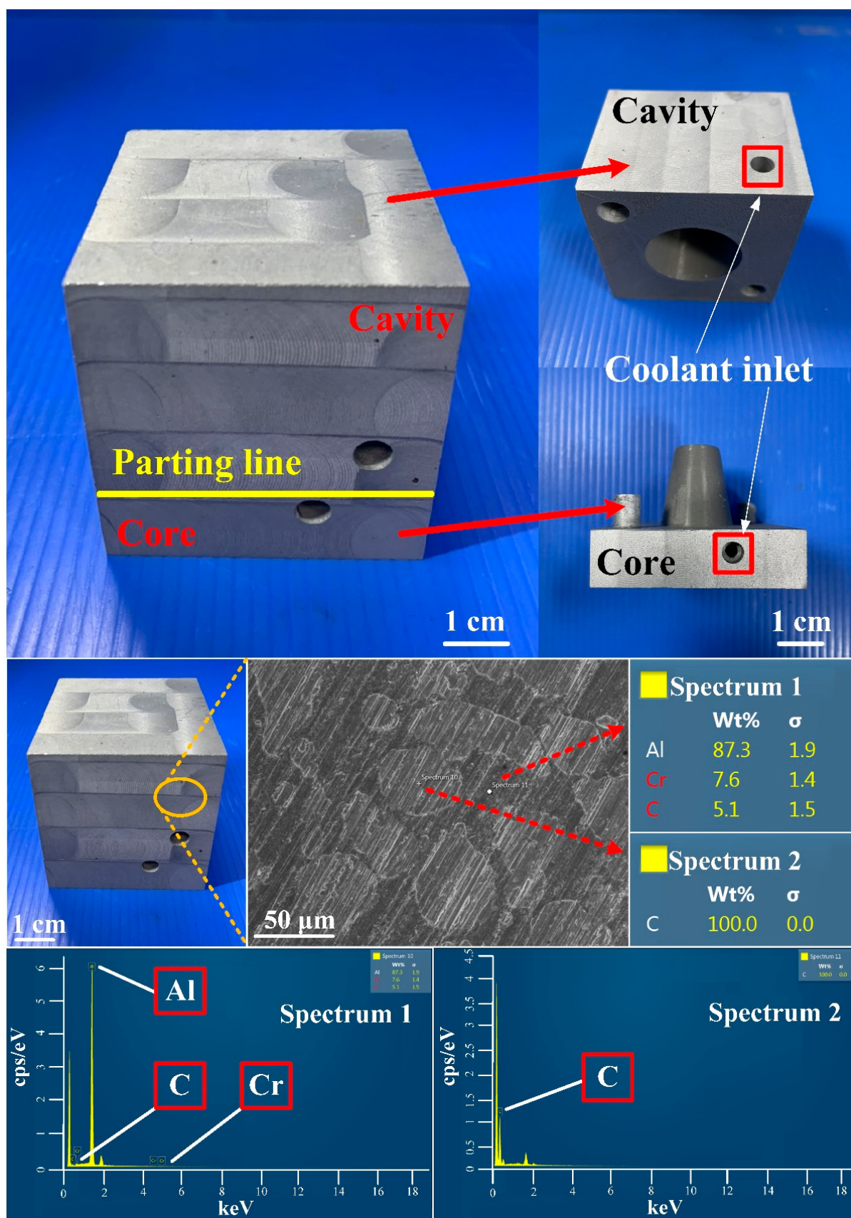
Figure 19. SEM micrographs and chemical composition of wax injection mold fabricated by epoxy resin added with 39 vol.% Al powder.
