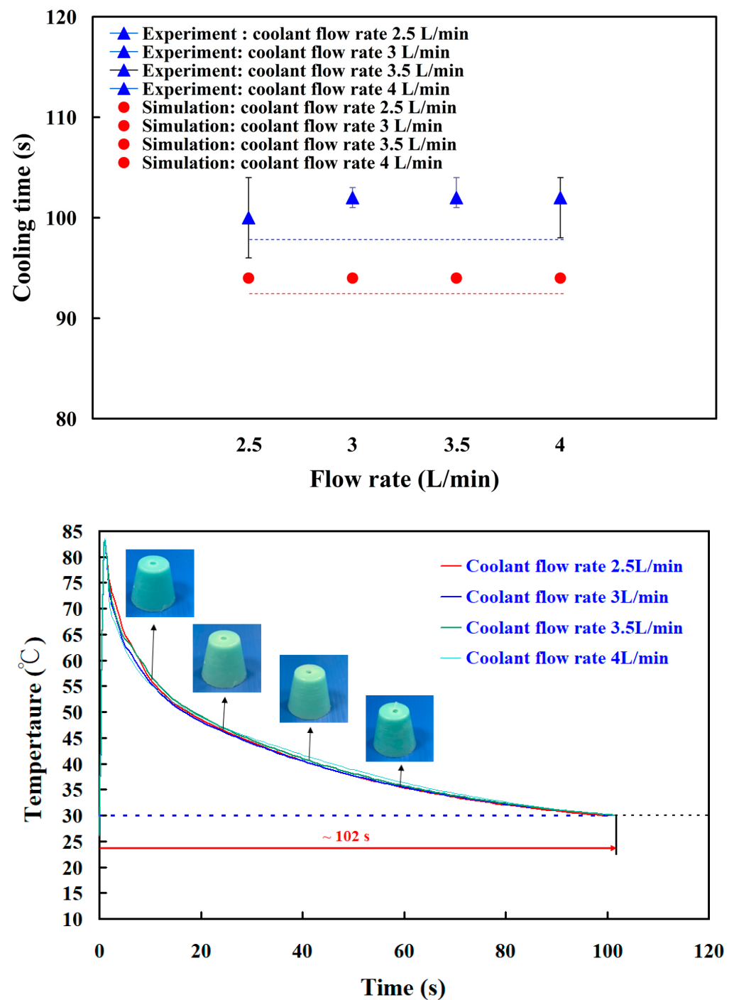
Figure 24. The cooling time of the wax pattern as a function of flow rate.
