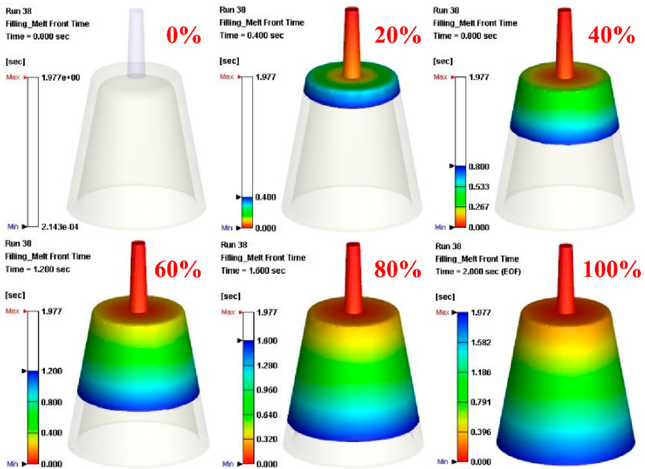
Figure 12. Filling time of the injection-molded part.
