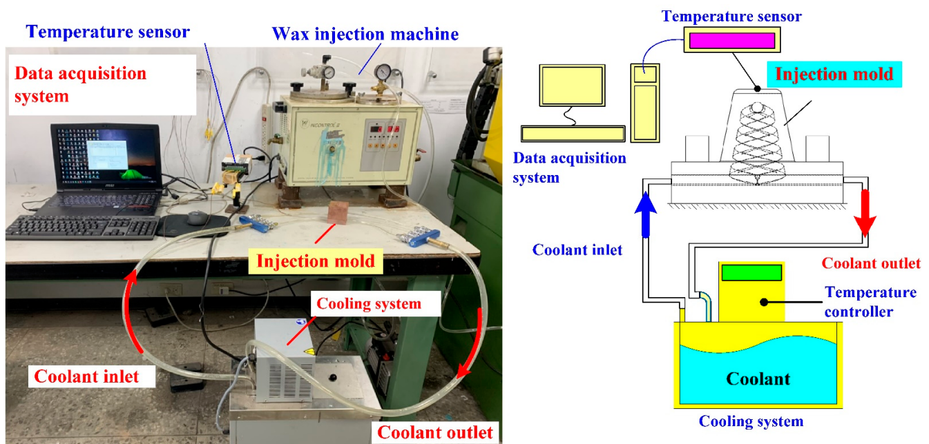
Figure 9. An in-house cooling time measurement system.
