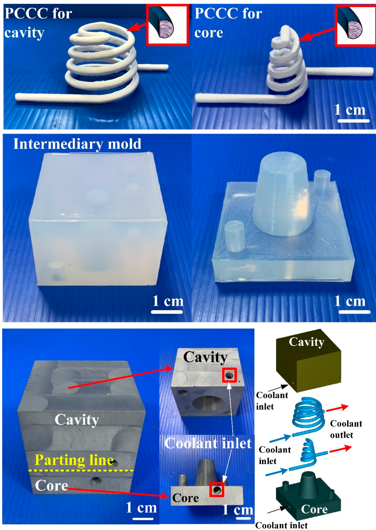
Figure 16. Injection mold fabricated with commercial material.
