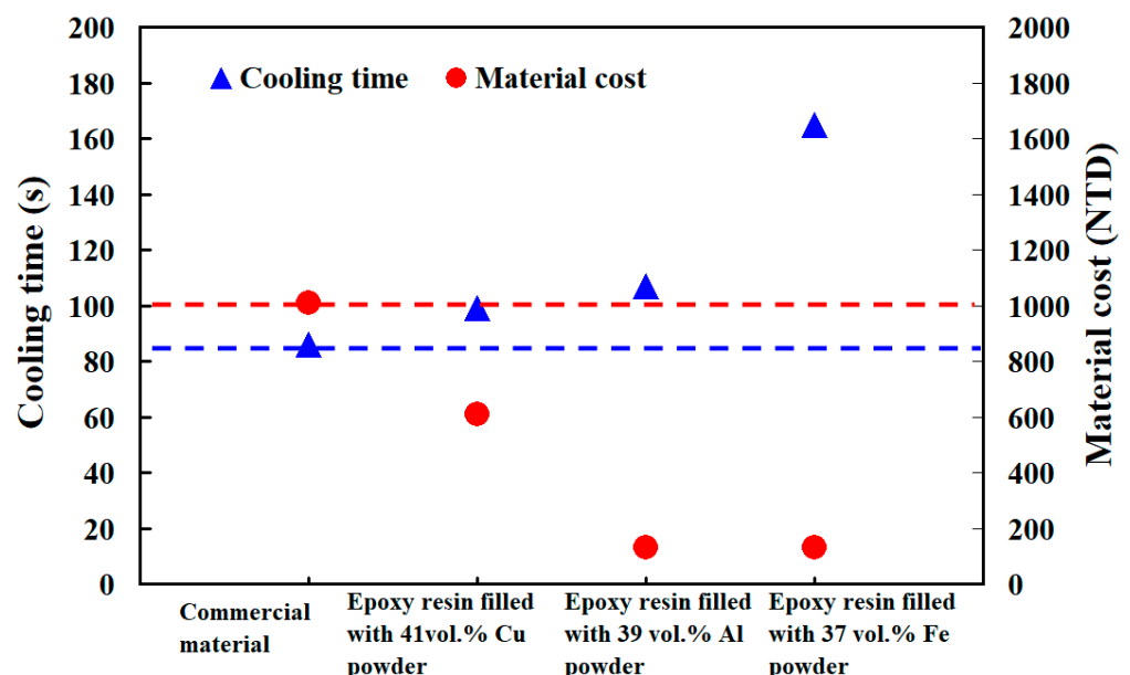
Figure 25. Four different kinds injection molds of material cost and cooling time of the wax pattern.
