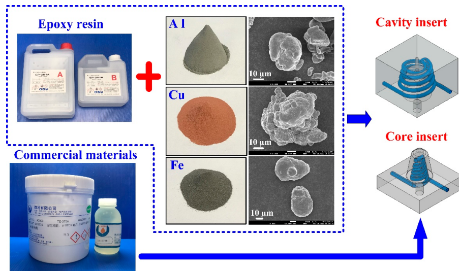
Figure 4. Three different kinds of fillers were added into the epoxy resin to make injection molds.
