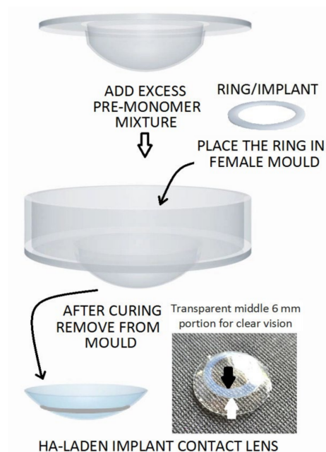
Figure 3. Proposed HA-laden embedded contact lens with a modified cast-molding method (the white arrow indicates the outer margin and the black arrow indicates the inner margin of the ring implant). With permission ©2017, Acta biomaterialia.
