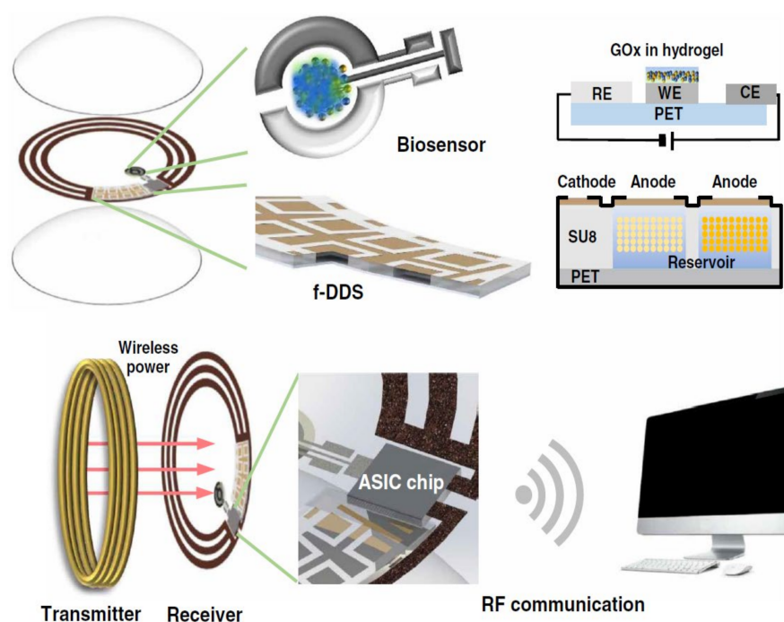
Figure 2. Remotely controllable smart contact lens designed for noninvasive glucose measurement and controlled drug release targeting diabetic retinopathy. With permission ©2020, Science Advances.
