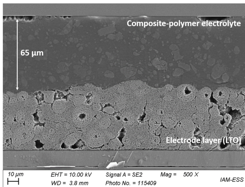
Figure 6. Scanning electron microscope image of the cross-section of a polymer electrolyte coated LTO electrode; 500× magnification.
