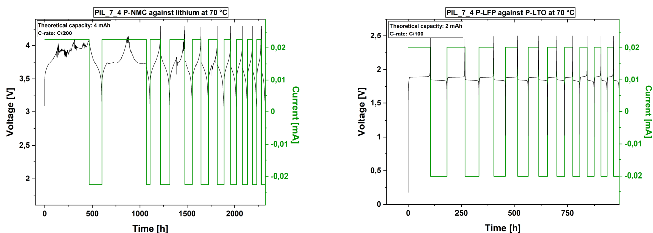
Figure 7. First 10 cycles of the cell test of the polymer electrolyte with MPPyrr-TFSI to EC ratio of 1:1 (PIL_7_4) at 70 °C with the electrode combinations NMC111 against lithium ( left ; C/200) and lithium iron phosphate against lithium titanate ( right ; C/100). Images including all executed cycles are given in the Supporting Material section (Figure S5).
