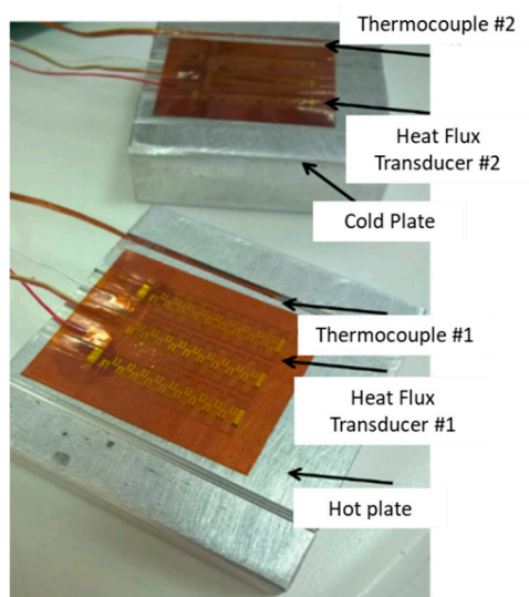
Figure S1. Apparatus for the measurement of thermal conductivity
