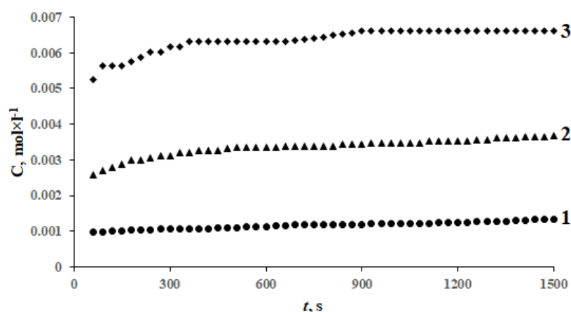
Figure 1. Kinetic curves of methylene blue polymerization at the following temperatures: 1–298 K; 2–308 K; 3–318 K (methylene blue concentration 5 \times 10^{-3} \text{ mol} \times \text{L}^{-1} ; concentration of ammonium peroxodisulfate 0.02 \text{ mol} \times \text{L}^{-1} ).
