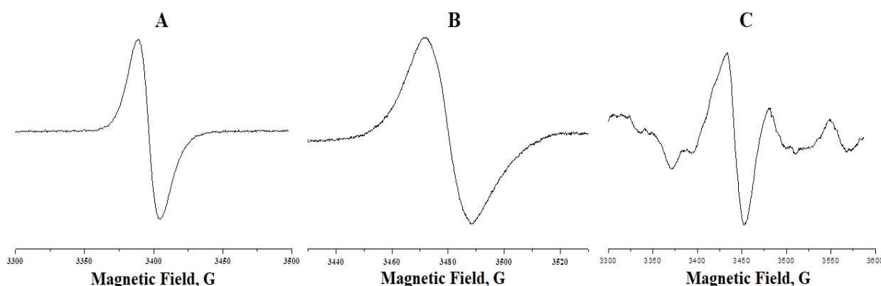
Figure 6. EPR spectra: (A)—methylene blue; (B)—polymethylene blue washed with five portions of distilled water, 100 mL each; (C)—washed with 25 portions of distilled water, 100 mL each.
