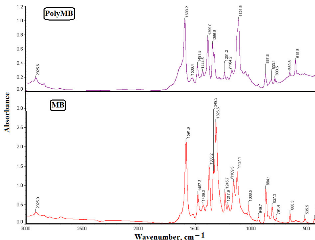
Figure 8. IR spectra: MB—methylene blue; PolyMB—polymethylene blue, recorded in potassium bromide tablets.
