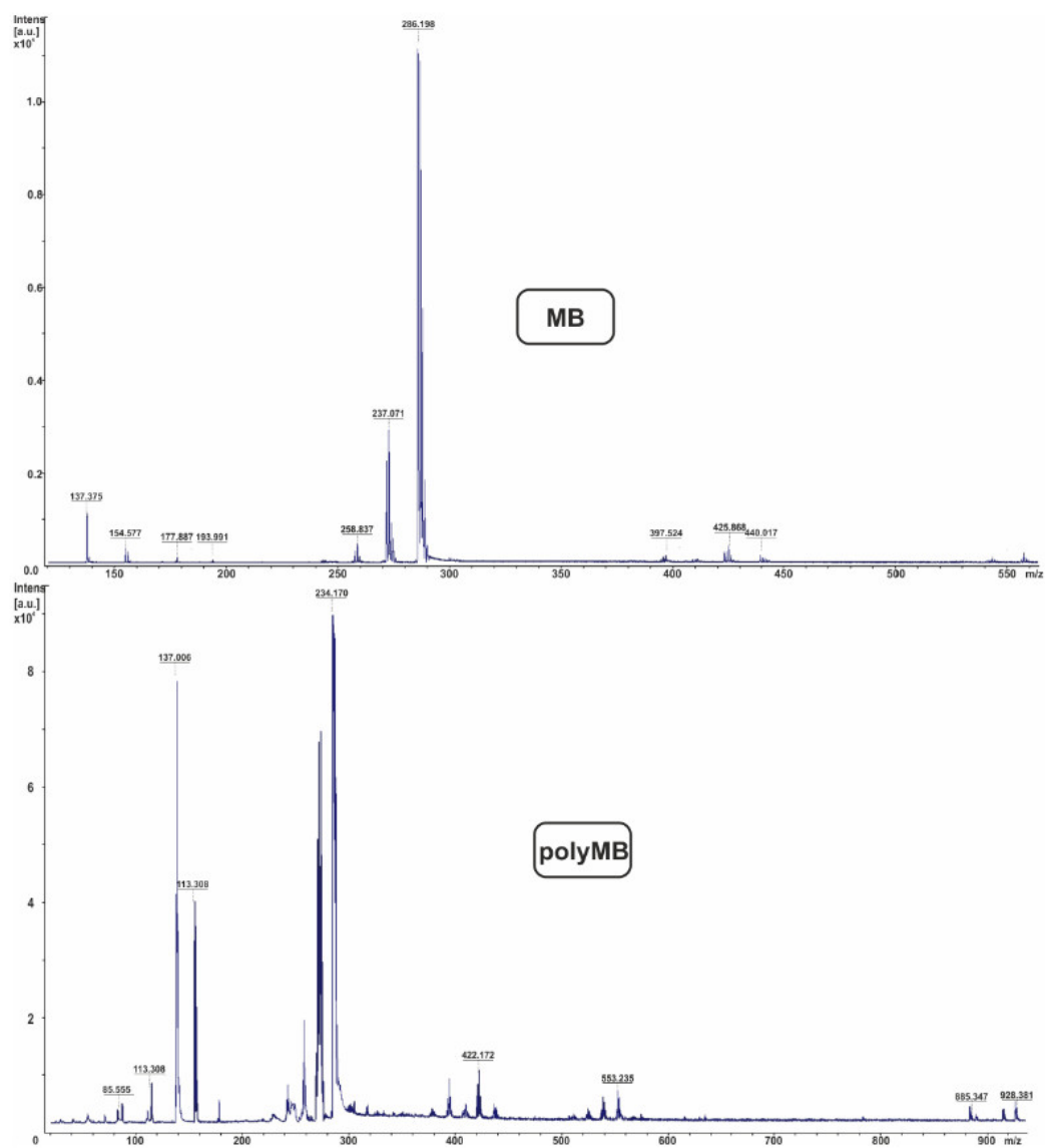
Figure 4. Spectra MALDI: MB—methylene blue; PolyMB—polymethylene blue.
