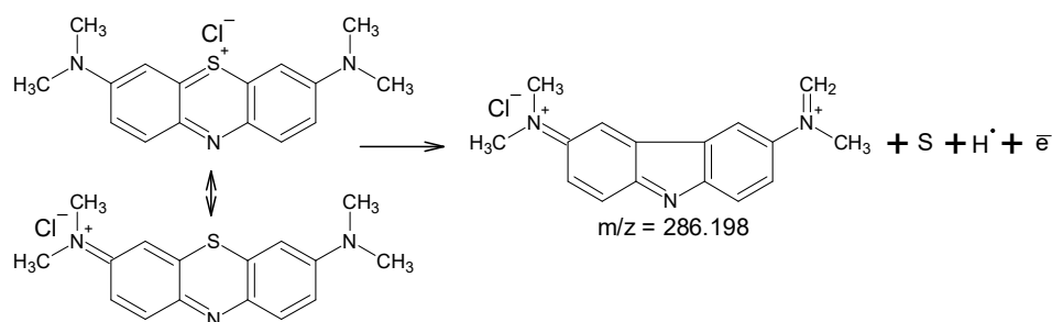
Scheme 4. Destruction of methylene blue under conditions of laser desorption from a DHB matrix.
