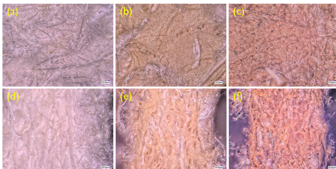
Figure 9. Focus stacked images of the surface and cross-section for (a, d) R-RM nonwoven, (b, e) R-RM nonwoven dyed at 100 °C, and (c, f) R-RM nonwoven dyed at 140 °C.
