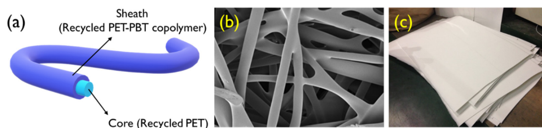
Figure 2. (a) Schematic illustration of the recycled bicomponent polyester filament fiber, (b) scanning electron microscope image (mag. ×300), and (c) photograph of the thermal-bonded nonwoven (R-RM nonwoven) formed therefrom.
