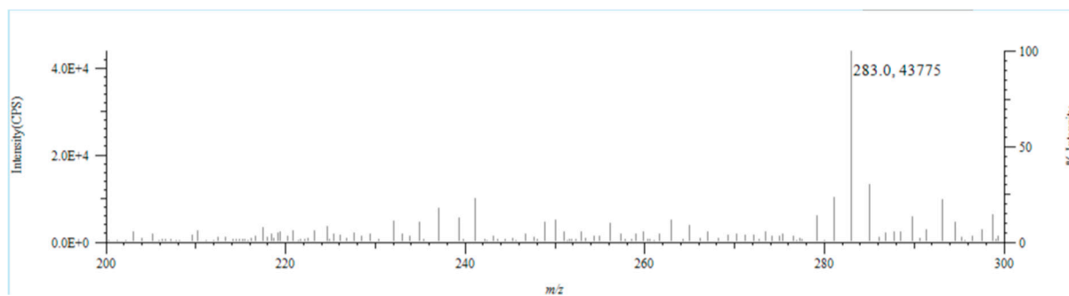
Figure S4. Mass spectrum of Cys-NAC disulfide determined by LC-MS with positive ESI mode
