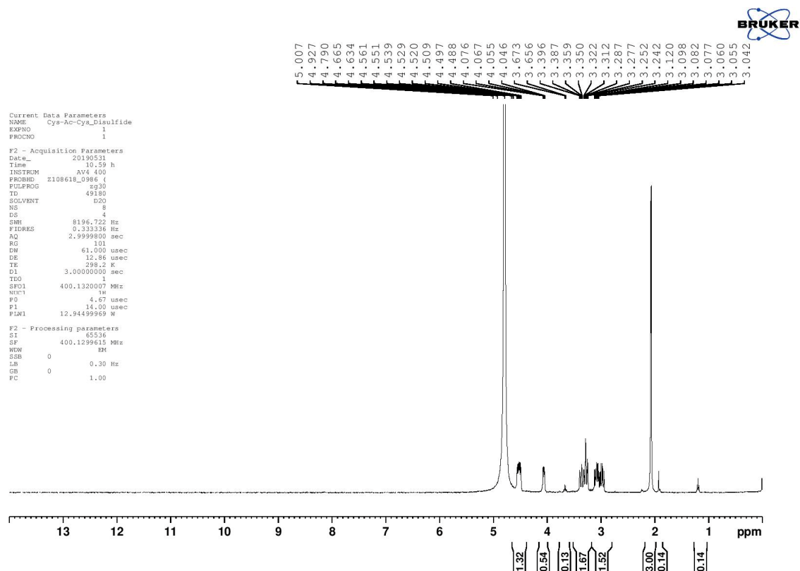
Figure S3. ^1\text{H} -NMR spectrum of Cys-NAC
