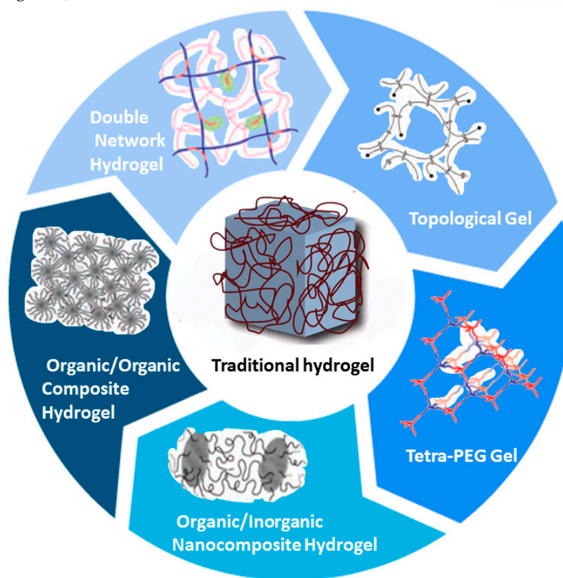
Figure 1. Typical network structures of traditional and several high-strength hydrogels [12].
