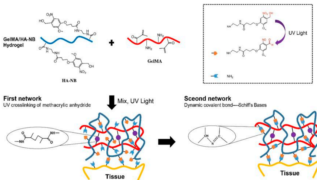
Figure 6. Constituent chemical structures and a schematic diagram illustrating the formation of the photo-triggered imine-crosslinked matrix hydrogel. The effective wet-adhesion properties of the matrix gel derive from photo-generated aldehyde groups bonding with the amino groups on the tissue surface and its mechanical strength derives from its two internal covalently crosslinked networks. Upon UV irradiation, the methyl methacrylate-modified gelatin (GelMA) rapidly generates the first crosslinked network elements of the hydrogel. Meanwhile, some of the photo-generated aldehyde groups on the o-nitrobenzyl-based modified hyaluronic acid (HA-NB) at the tissue–hydrogel interface react with amino groups of the tissue proteins and proteoglycans, forming Schiff bases. Meanwhile, the photo-generated aldehyde groups on the hydrogel HA-NB react with the amino groups of GelMA to form a second crosslinking network. As the reaction progresses, the remaining aldehyde groups react with amino groups of the tissue and GelMA to bond tissue and increase internal crosslinking. The creation of two different chemically crosslinked matrices lead to a significant increase in the tissue adhesion and internal strength of the hydrogel. The good wet tissue adhesion and mechanical properties of the hydrogel would ensure its stability in wound closure [76,79].
