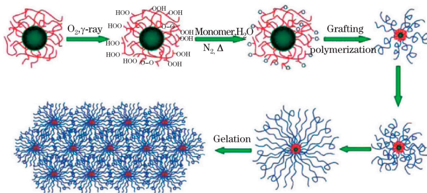
Figure 3. Proposed mechanism for formation of macromolecular microsphere composite (MMC) hydrogel and MMC hydrogel microstructure [28].
