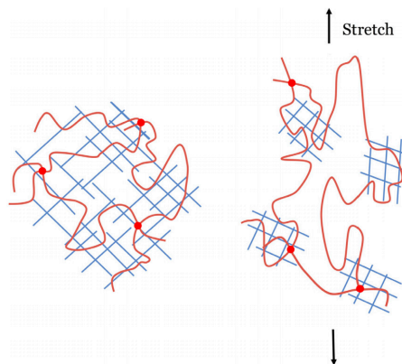
Figure 2. A double-network hydrogel consists of two polymer networks: a short-chain network that can swell nearly to the breaking point, and a long-chain network that is highly stretchable. When the hydrogel is stretched, the short-chain network ruptures, but the long-chain network remains elastic [18].
