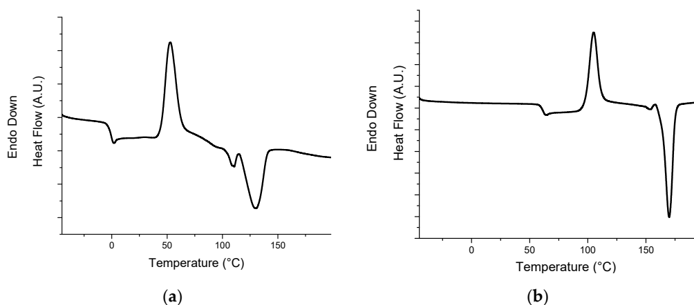
Figure 2. DSC thermograms recorded during the second heating scan for virgin (a) PHB and (b) PLA.
