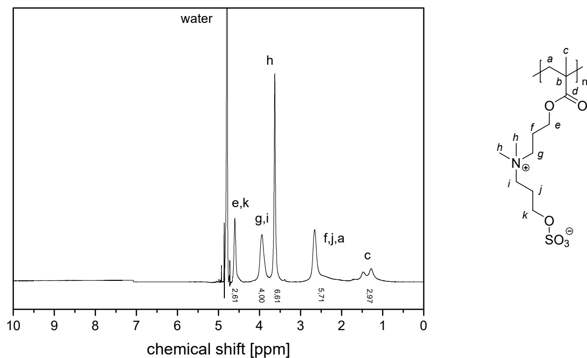
Figure A14. ^1\text{H} NMR-spectrum of polymer P-2d in \text{D}_2\text{O} saturated with NaCl.
