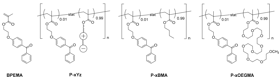
Figure 3. Chemical structure of the photo-reactive comonomer BPEMA used, the photo-crosslinkable copolymers P-xYz (with Y = 1–6 and z = a–d; see also Figure 1), and of the reference copolymer systems P-xBMA and P-xOEGMA.
