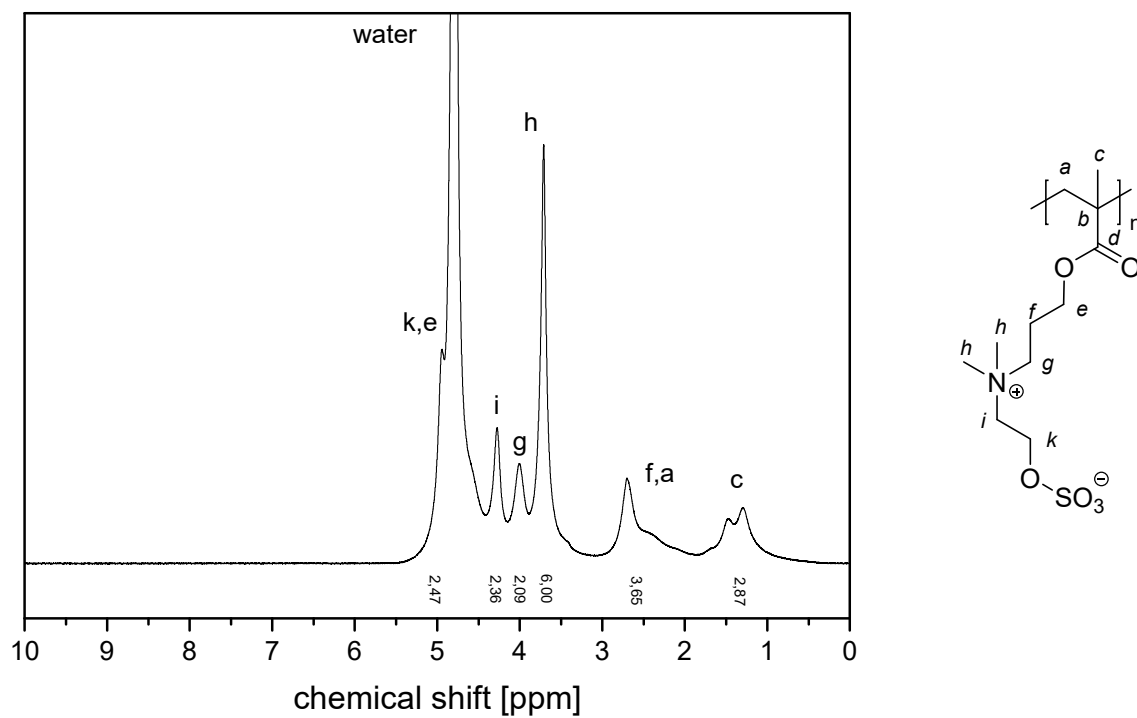
Figure A13. ^1\text{H} NMR-spectrum of polymer P-2c in \text{D}_2\text{O} saturated with NaCl.
