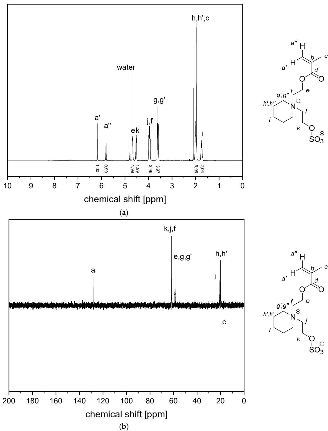
Figure A5. (a) ^1\text{H} NMR- spectra and (b) ^{13}\text{C} (APT) NMR-spectra of monomer 4c in \text{D}_2\text{O} .
