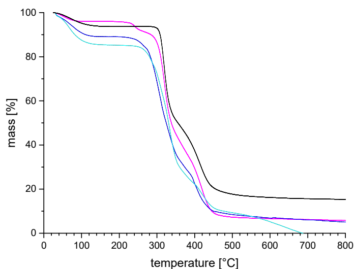
Figure 2. Exemplary TGA thermograms of zwitterionic polymer series P-4: (—) = P-4a; (—) = P-4b; (—) = P-4c; (—) = P-4d.
