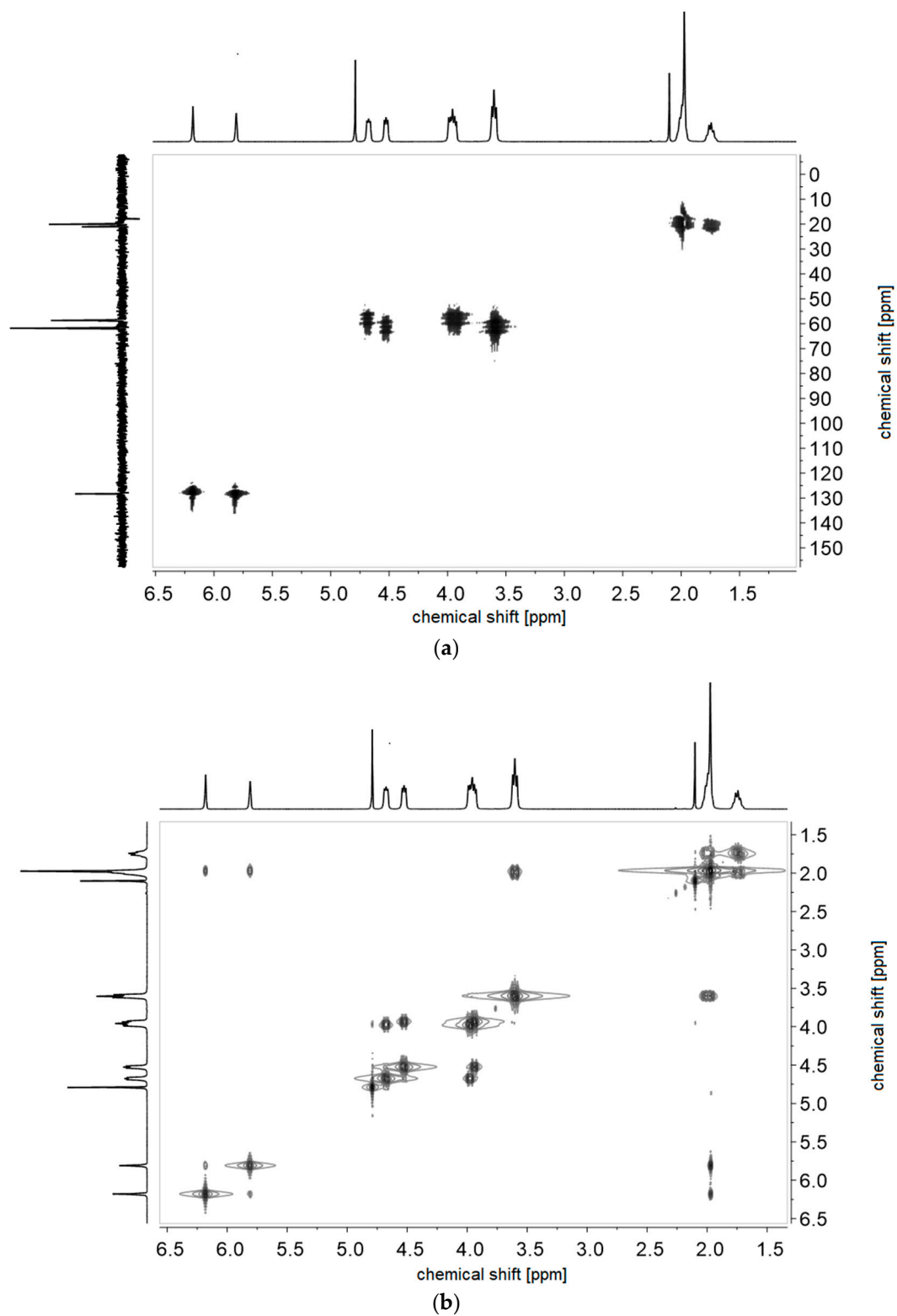
Figure A6. (a) 1 H- 1 H-COSY- and (b) 1 H- 13 C-HMQC NMR-spectra of monomer of 4c in D 2 O.
