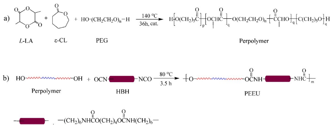
Figure S1. The reaction scheme of PEEU
