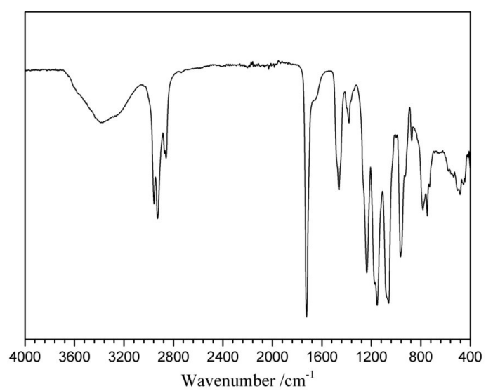
Figure S6. FT-IR spectrum of PME H
