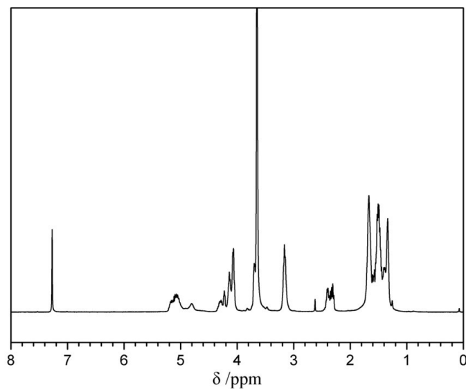
Figure S2. 1 H NMR spectrum of PEEU
